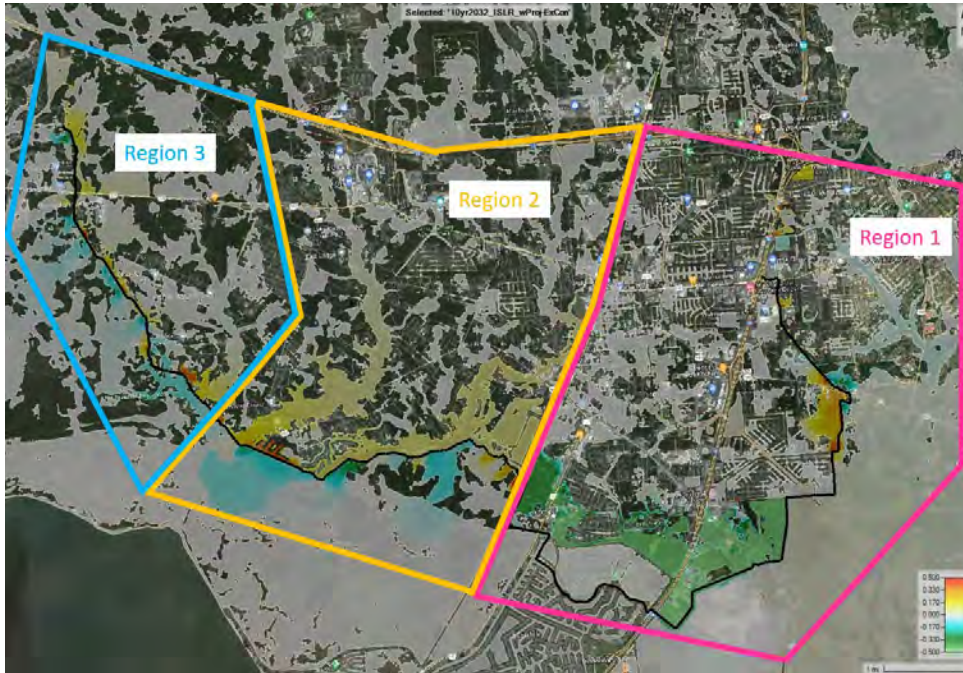
Figure E:14-7. 10-year 2032 event difference map depicting WSE increases and lowering's for the intermediate rate of SLR and coincident Frequency inflows on the Bogue Chitto River and Pearl River. Regions correlate to areas discussed in the following results section. For a comprehensive description of difference maps refer to Annex 3 of this appendix.
