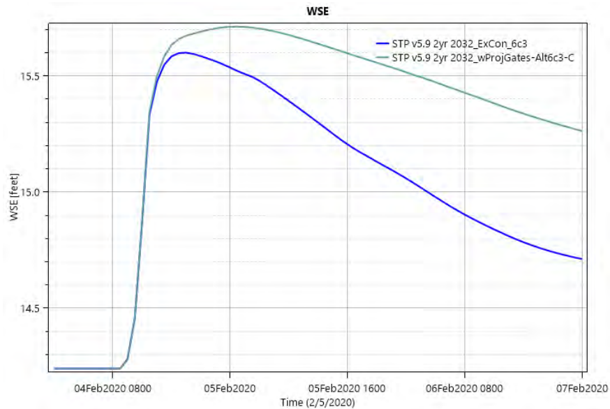
Figure E6:17. Point ID 16 - Pine Hardwood. Point is located on the protected side of the alignment North of the Hwy 190 embankment. WSE remains elevated through the end of the simulation because the highway embankment and levee interface create a pocket where water can pool.
