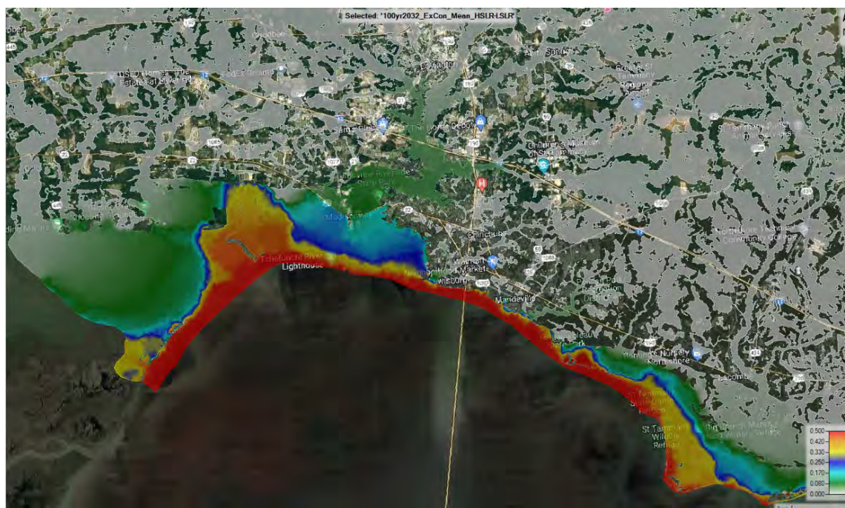
Figure E3:75. 100-year 2032 existing condition HSLR minus LSLR
