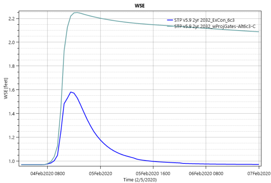
Figure E6:9. Point ID 8 - Pine Savannah. Point is located on the flood side of the alignment West of the Norfolk Southern Railroad. Water in this area moves from South to North and flows into Bayou Bonfouca. WSE remains elevated near the end of the simulation because the levee is obstructing the existing drainage path of water, forcing it to pool on the flood side of the alignment.
