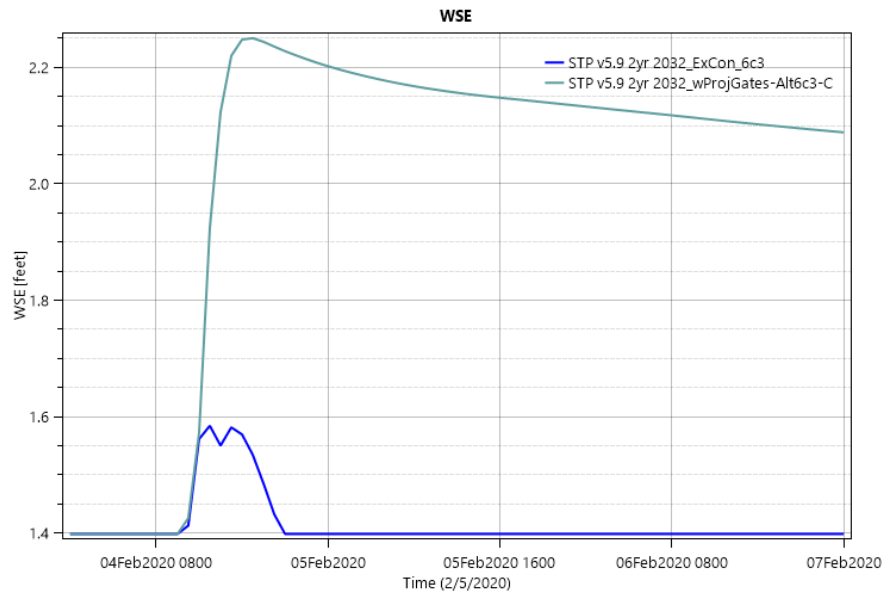
Figure E6:8. Point ID 7 - Pine Savannah. Point is located on the flood side of the alignment West of the Norfolk Southern Railroad. Water in this area moves from South to North and flows into Bayou Bonfouca. WSE remains elevated near the end of the simulation because the levee is obstructing the existing drainage path of water, forcing it to pool on the flood side of the alignment.
