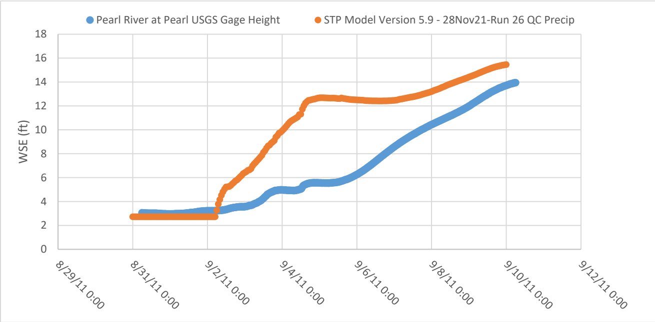
Figure E4:7. September 2011 calibration event plot for USGS Gage -Pearl River at Pearl, LA
