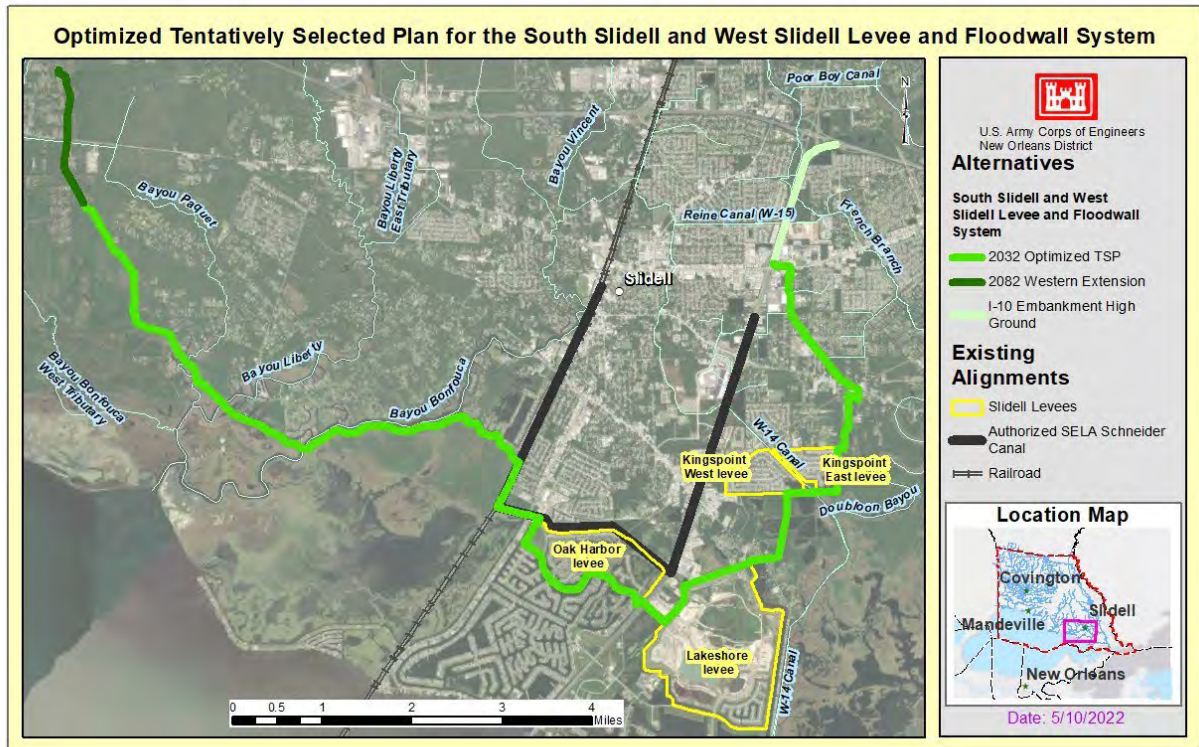
Figure E:14-5. Optimized TSP for the South Slidell and West Slidell Levee and Floodwall System
