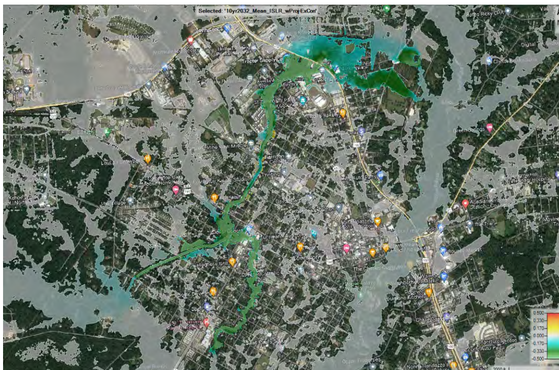
Figure E3:39. 10-year 2032 ISLR difference in WSE with project
