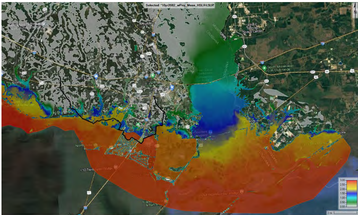
Figure E3:70. 10-year 2082 with-project HSLR minus LSLR
