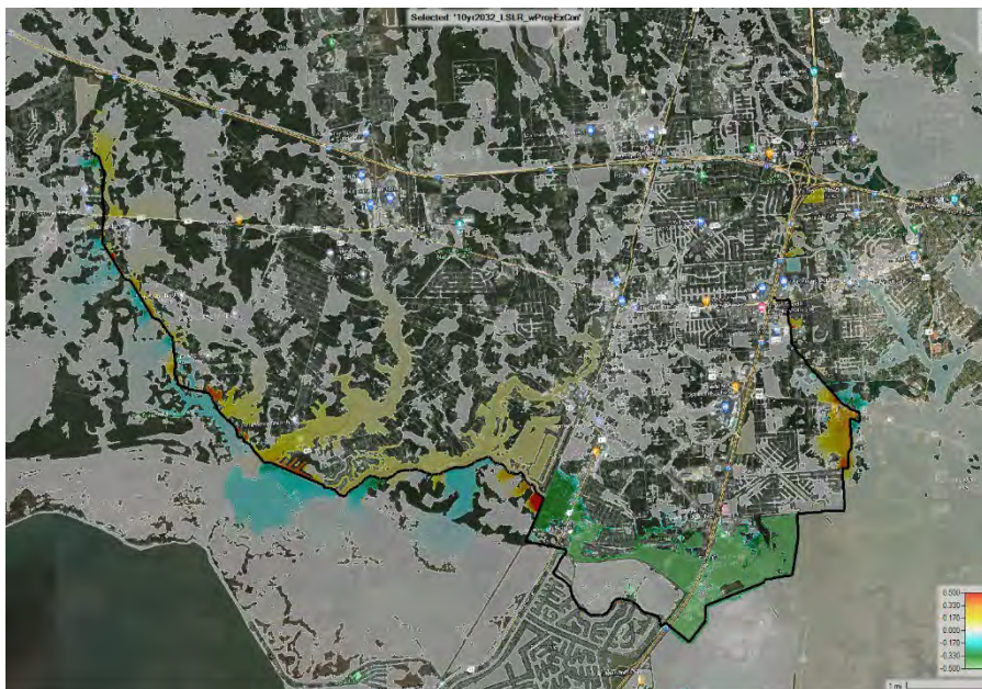
Figure E3:1. 10-year 2032 LSLR difference in WSE with project
