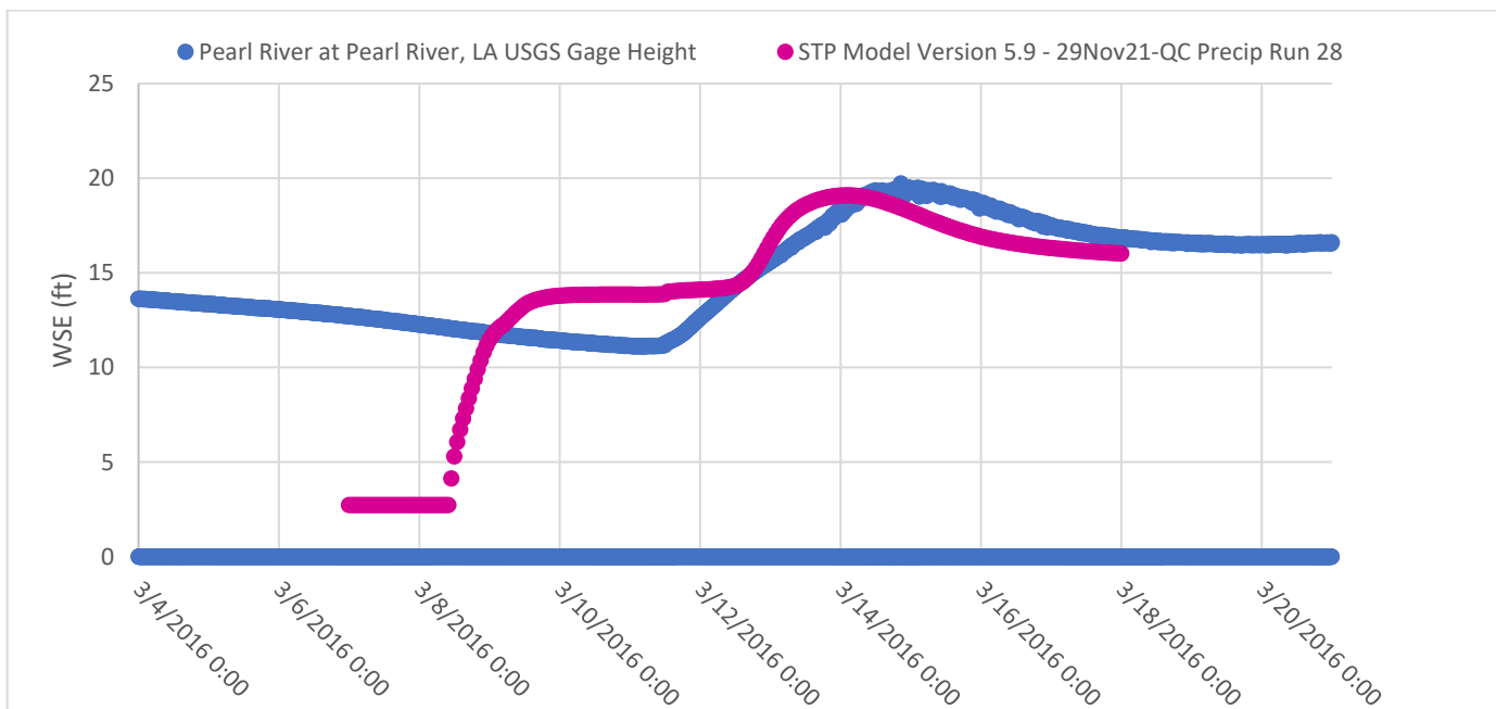
Figure E4:16. March 2016 calibration event plot for USGS Gage – Pearl River at Pearl, LA
