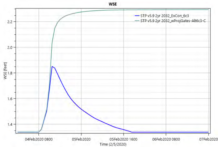
Figure E6:4. Point ID 3 - Pine Savannah. Point is located on the flood side of the alignment West of the Norfolk Southern Railroad. Water in this area moves from South to North and flows into Bayou Bonfouca. WSE remains elevated near the end of the simulation because the levee is obstructing the existing drainage path of water, forcing it to pool on the flood side of the alignment.
