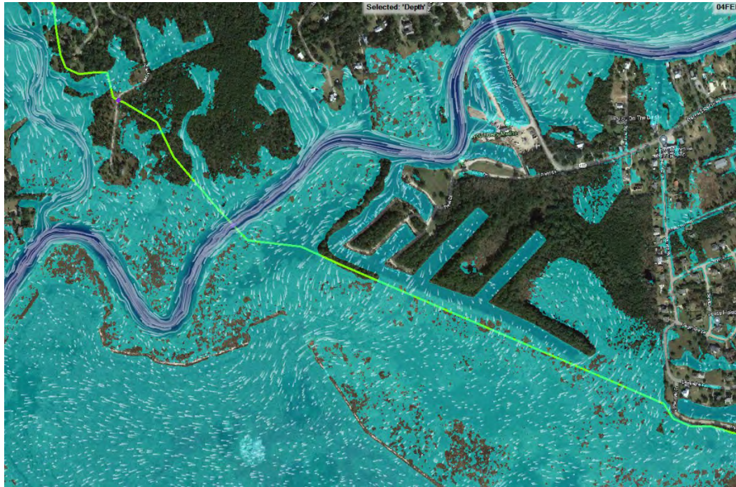
Figure E5:14. Segment 5 Existing Conditions
