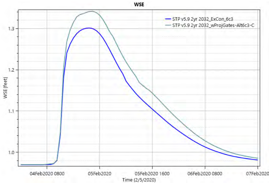
Figure E6:12. Point ID 11 - Intermediate Marsh. Point is located on the protected side of the alignment on the right descending bank of Bayou Liberty approximately 0.4miles upstream of the gate crossing. WSE returns near pre-project levels by the end of the simulation.
