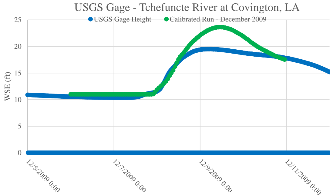
Figure E2:16. December 2009 calibration event plot for USGS Gage -Tchefuncte River at Covington, LA
