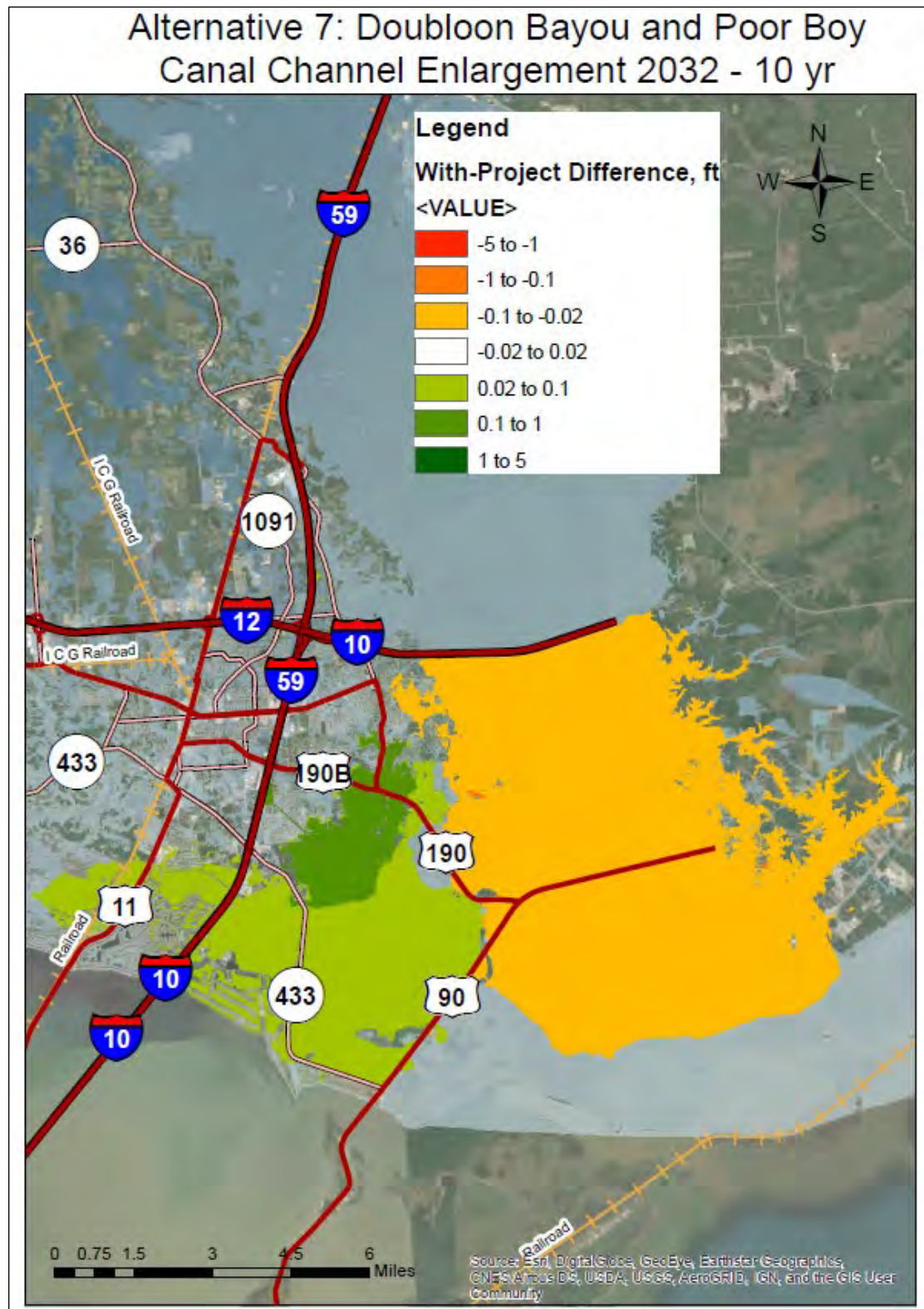
Figure E1:7. Baseline Conditions (year 2032) 10yr frequency event for Doubloon Bayou and Poor Boy Canal Channel Enlargements
