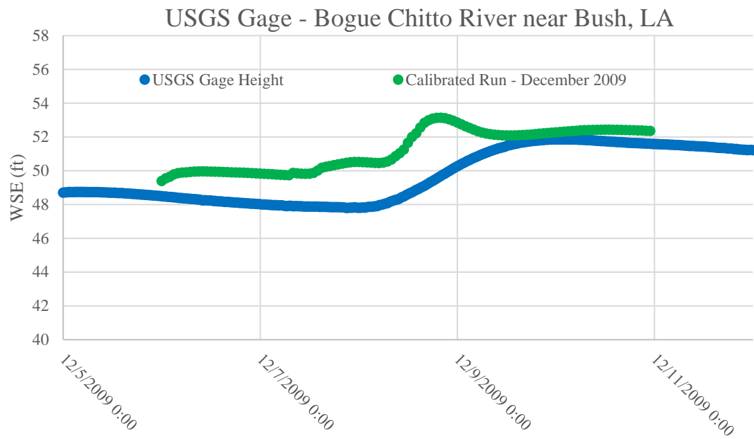
Figure E2:13. December 2009 calibration event plot for USGS Gage -Bogue Chitto River near Bush, LA
