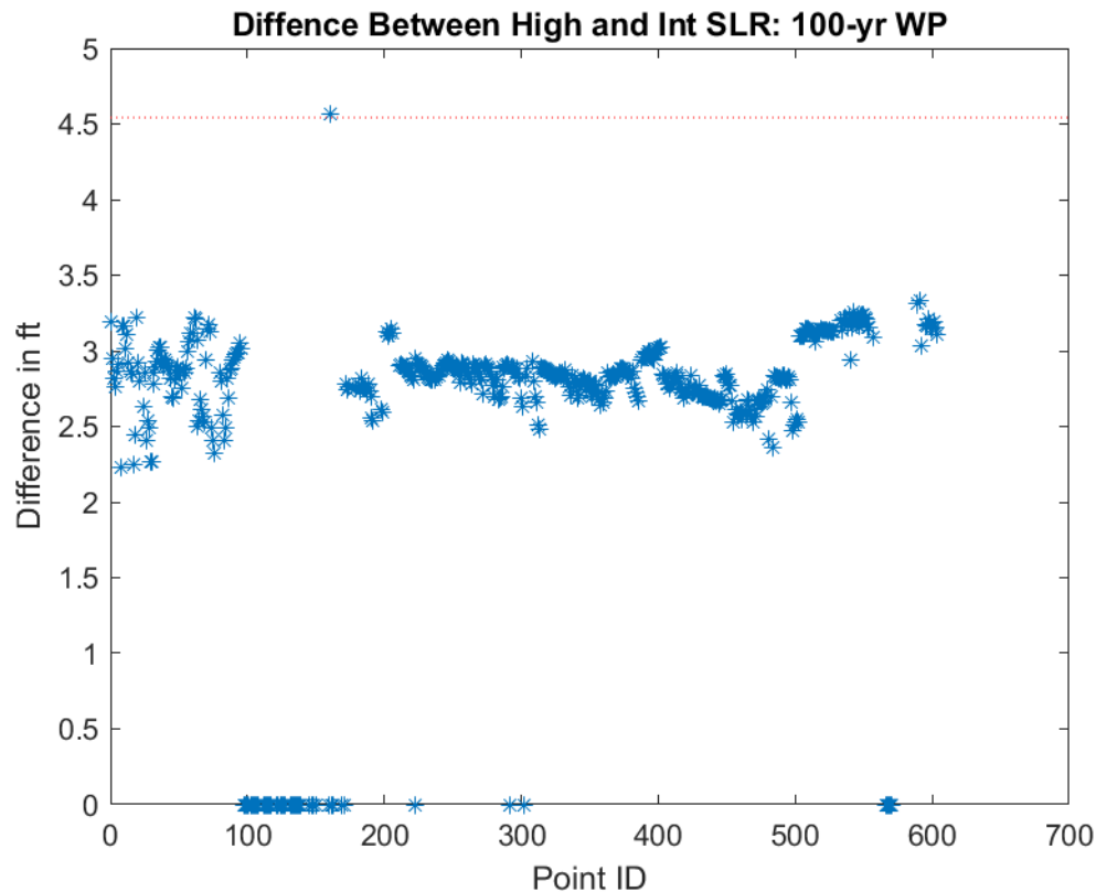
Figure E:13-14. Difference between extrapolated high SLR scenario WSE value and original future intermediate SLR value at a given location. Values of 0 denote locations within the project area where values remained dry during simulation.
