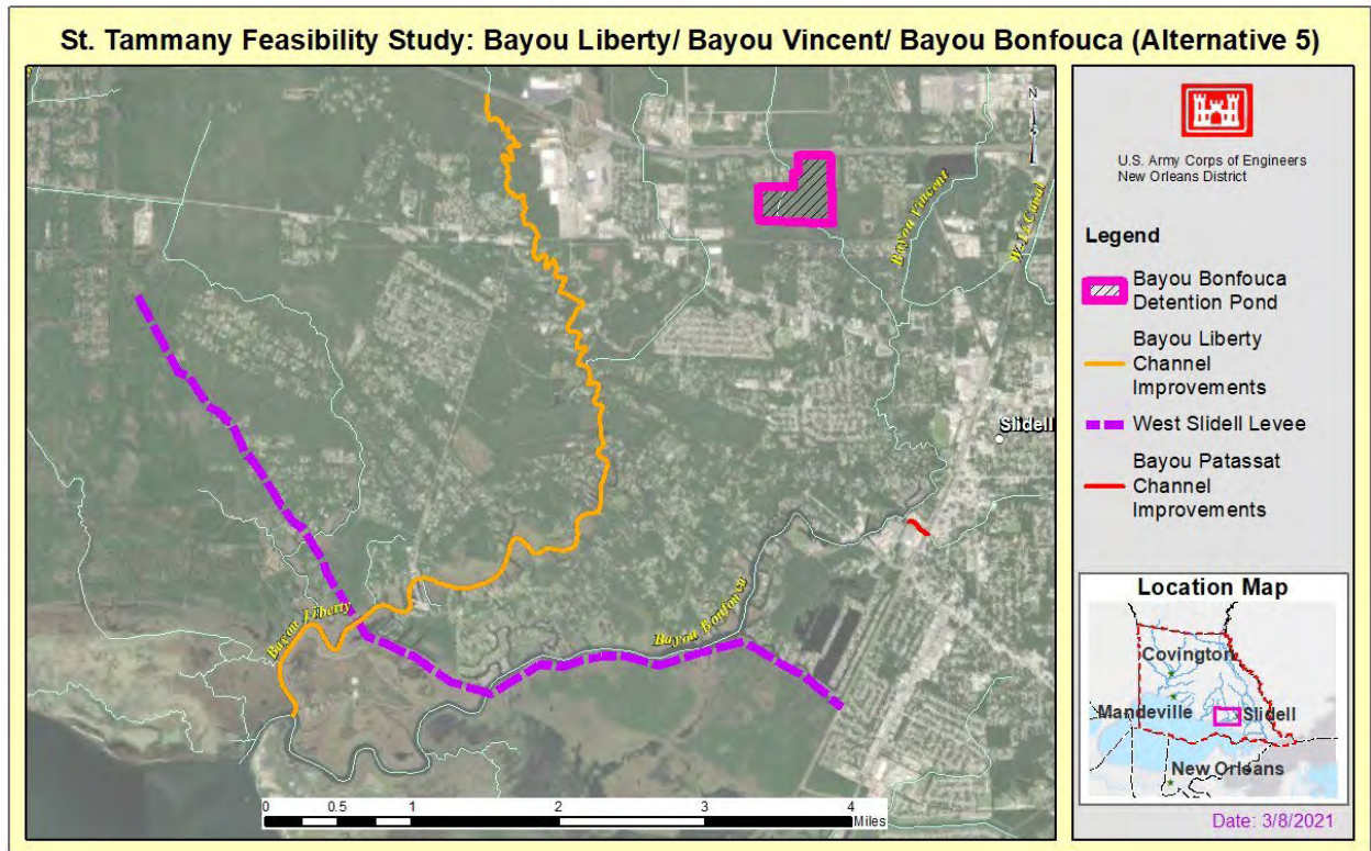
Figure E:6-12. Alternative 5 Measures: Bayou Bonfouca Detention Pond, Bayou Liberty Channel Improvements, West Slidell Levee, and Bayou Patassat Channel Improvements
