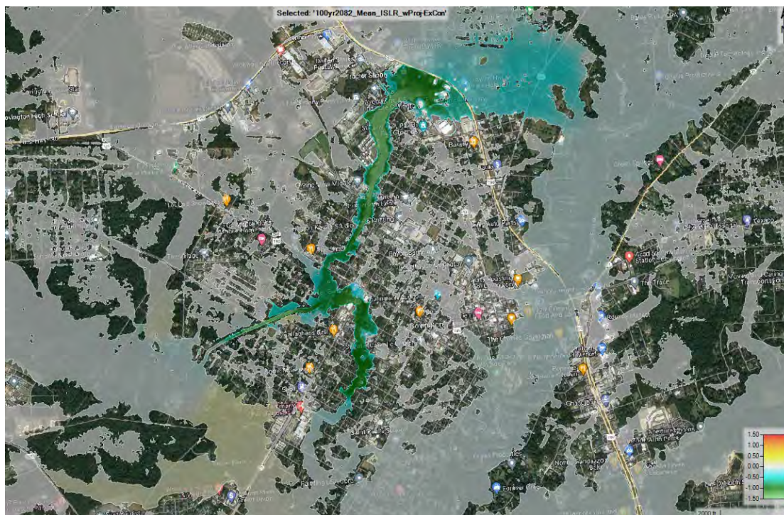
Figure E3:46. 100-year 2082 ISLR difference in WSE with project
