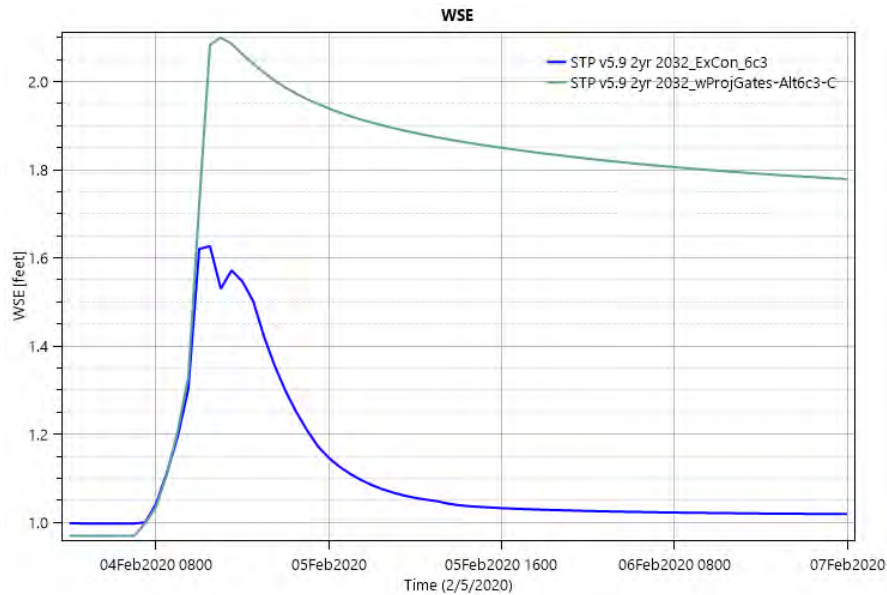
Figure E6:10. Point ID 9 - Pine Savannah. Point is located on the flood side of the alignment West of the Norfolk Southern Railroad and on the left descending bank of Bayou Bonfouca. Water in this location drains into Bayou Bonfouca. WSE remains elevated near the end of the simulation because the levee is obstructing the existing drainage path of water, forcing it to pool on the flood side of the alignment.
