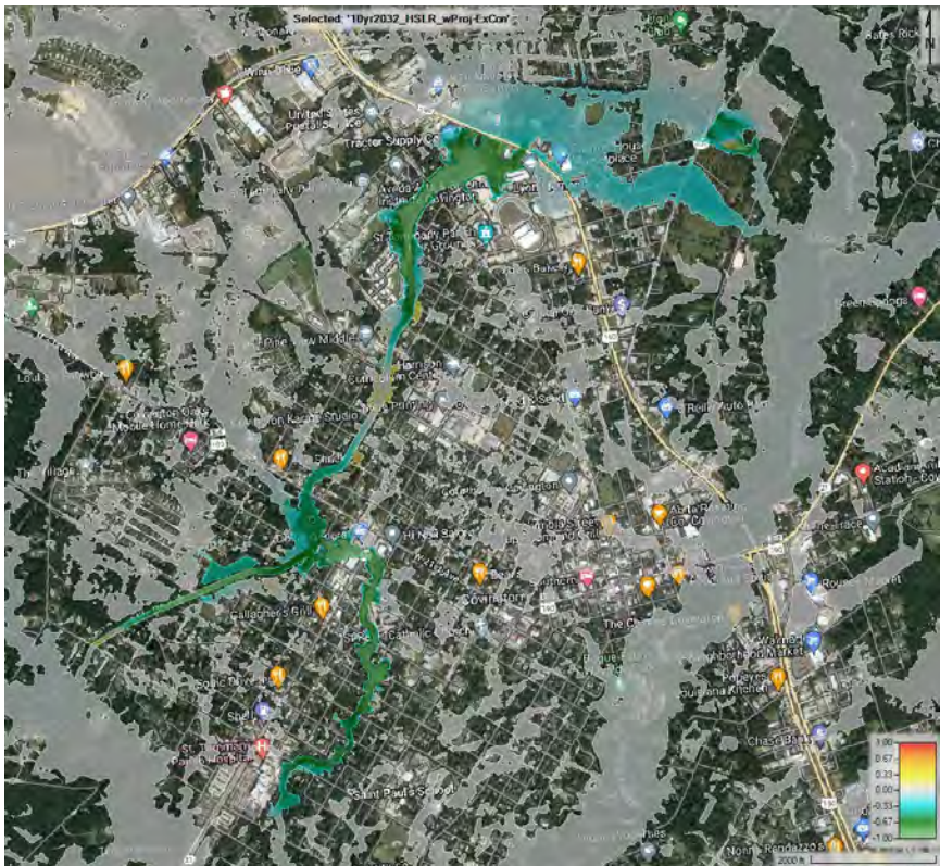
Figure E3:17. 10-year 2032 HSLR Difference in WSE with project
