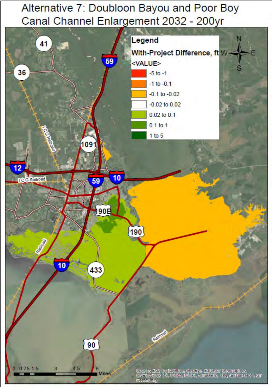
Figure E1:8. Baseline Conditions (year 2032) 200yr frequency event for Doubloon Bayou and Poor Boy Canal Channel Enlargements
