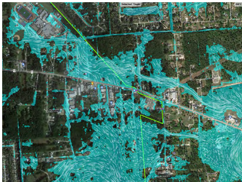
Figure E5:38. Segment 13 Existing Conditions
