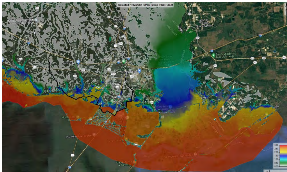
Figure E:14-11. 10-year 2082 event with-project HSLR-LSLR with mean inflows on the Pearl River and Bogue Chitto River
