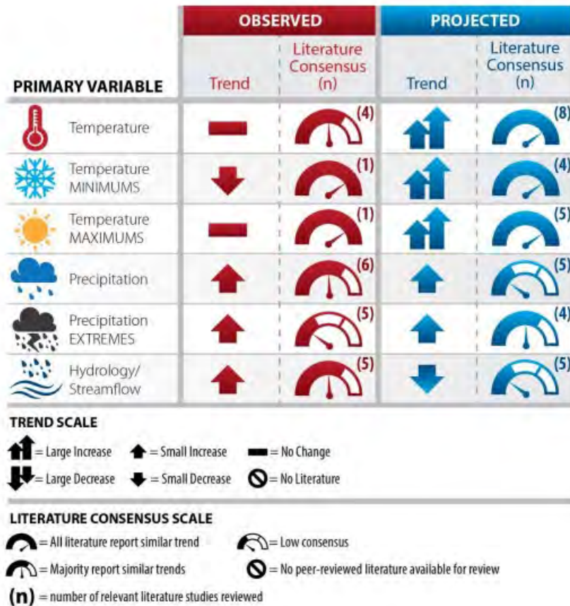
Figure E:11-6. Summary Matrix of Observed and Projected Climate Trends and Literary Consensus for Region 08 Source: U.S. Army Corps of Engineers (USACE 2015)
