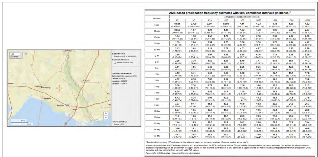
Figure E:3-2. Precipitation Frequency for Lacombe, LA (Central Location of the Parish)
