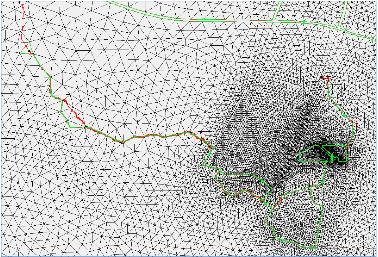
Figure E:13-12. ADCIRC mesh showing the levees/floodwalls as weir pairs (green) with the altered alignment (red)
