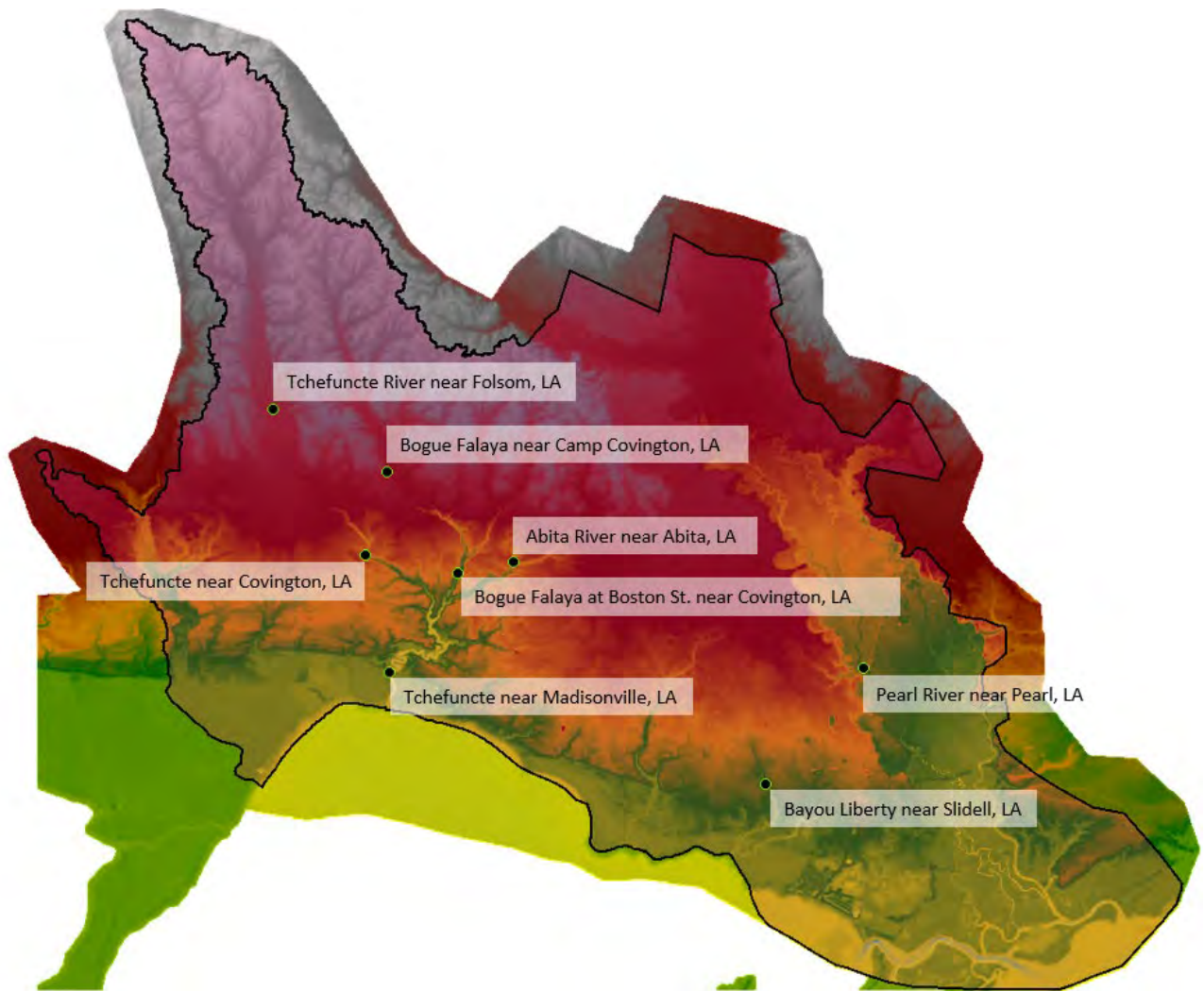
Figure E:12-5. Calibration Gage Locations for September 2011 and March 2016 Events
