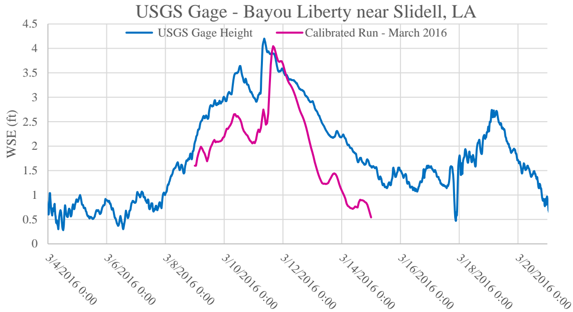
Figure E2:5. March 2016 calibration event plot for USGS Gage-Bayou Liberty near Slidell, LA
