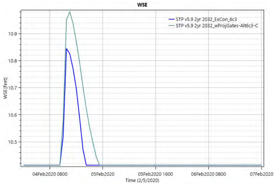
Figure E6:16. Point ID 15 - Pine Hardwood. Point is located on the protected side of the alignment South of the Tammany Trace trail. WSE returns to pre-project levels within 36 hours.
