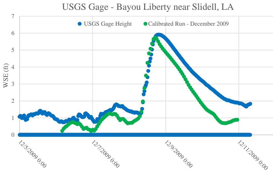
Figure E2:15. December 2009 calibration event plot for USGS Gage -Bayou Liberty near Slidell, LA
