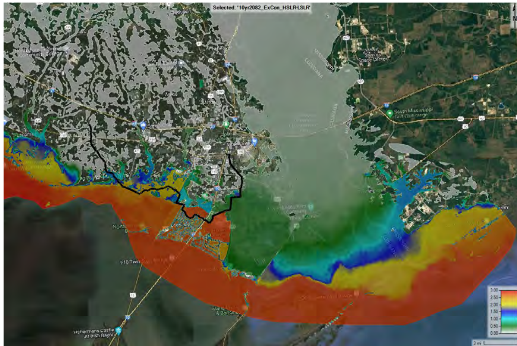
Figure E:14-8. 10-year 2082 event Existing Condition HSLR-LSLR with coincident frequency inflows on Pearl River and Bogue Chitto River
