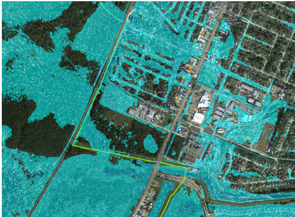
Figure E5:24. Segment 8 With Project
