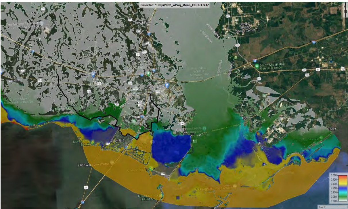
Figure E3:71. 100-year 2032 with-project HSLR minus LSLR
