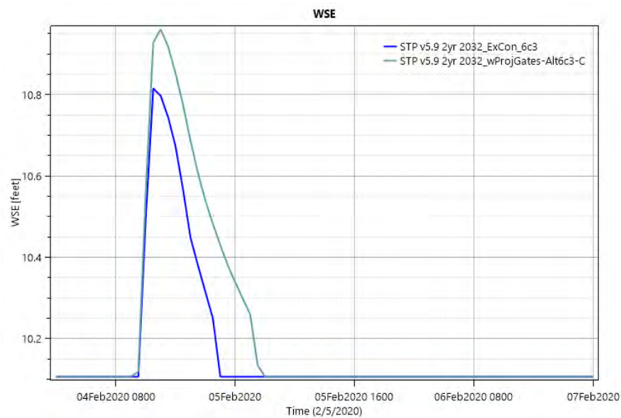
Figure E6:15. Point ID 14 - Pine Hardwood. Point is located on the protected side of the alignment near CC Road. WSE returns to pre-project levels within 36 hours.
