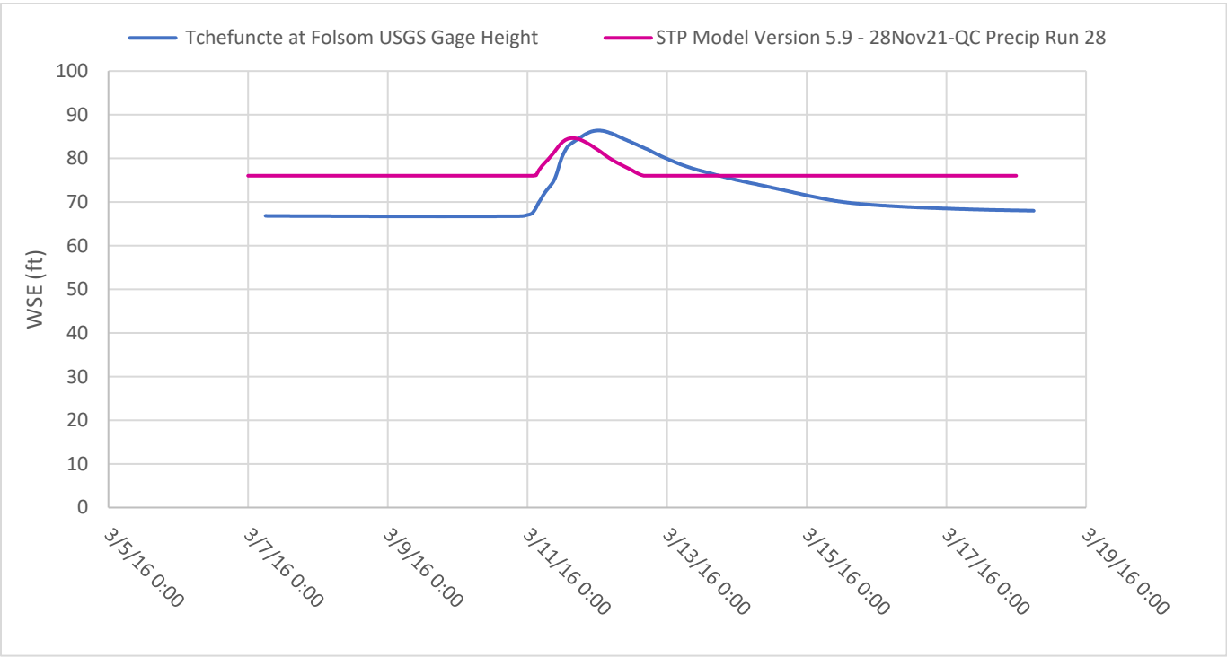
Figure E4:9. March 2016 calibration event plot for USGS Gage -Tchefuncte River at Folsom, LA
