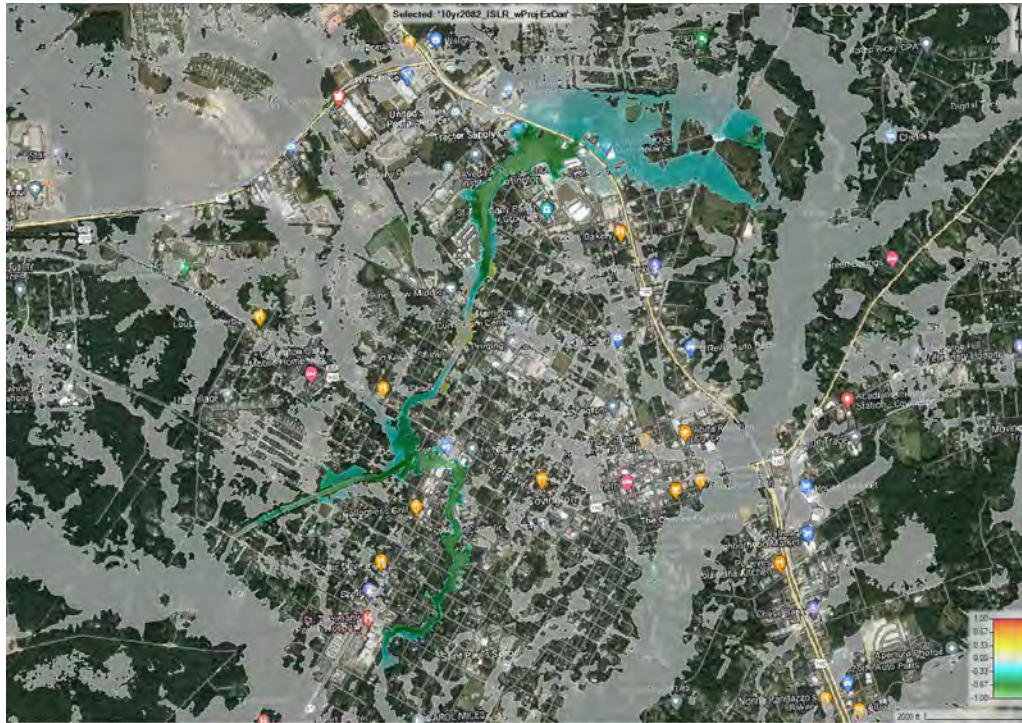
Figure E3:16. 10-year 2082 ISLR Difference in WSE with project
