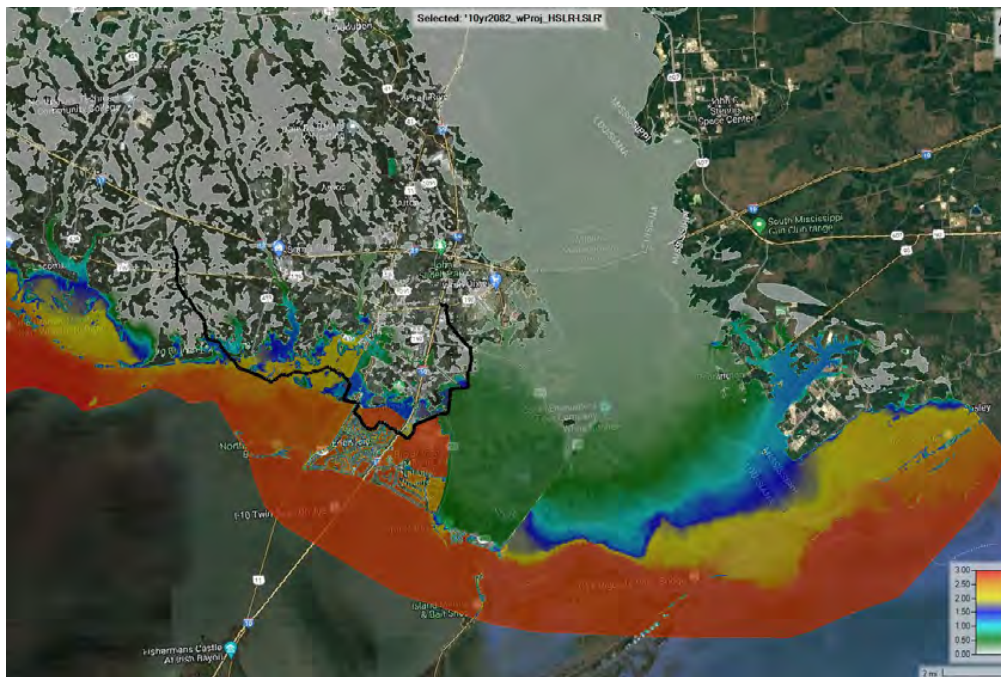
Figure E:14-9. 10-year 2082 event With-Project HSLR-LSLR with coincident frequency inflows on Pearl River and Bogue Chitto River
