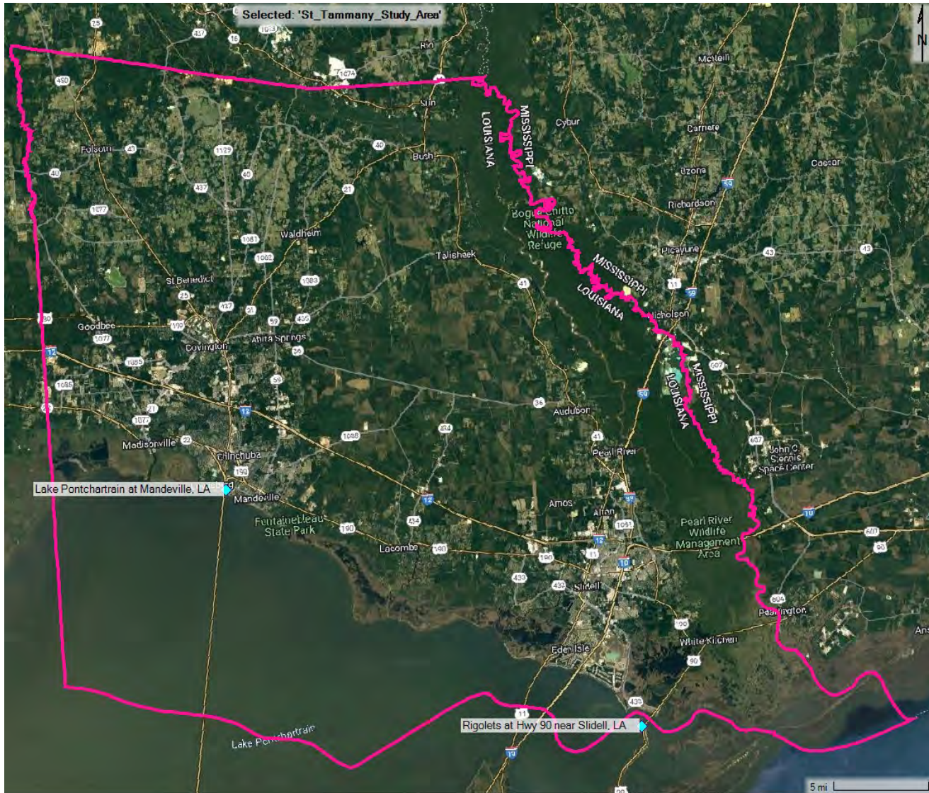
Figure E:11-3. St. Tammany Parish Extents and location of tide gages in Mandeville, LA and at the Rigolets near Slidell, LA.
