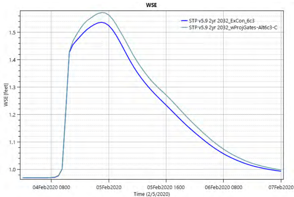
Figure E6:13. Point ID 12 - Intermediate Marsh. Point is located on the protected side of the alignment on the right descending bank of Bayou Liberty approximately 0.7miles upstream of the gate crossing. WSE returns to near pre-project levels by the end of the simulation.
