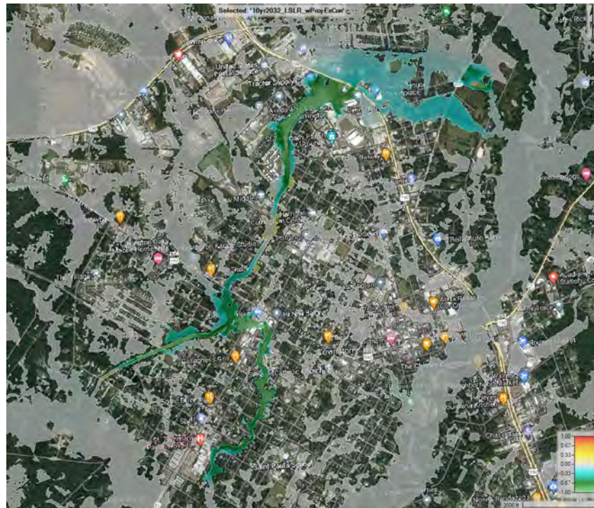
Figure E3:13. 10-year 2032 LSLR difference in WSE with project
