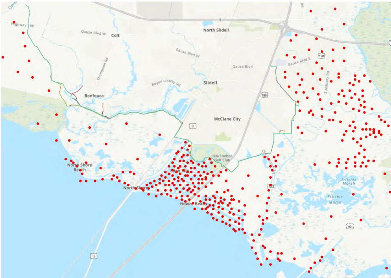
Figure E:13-13. Location of points where surge elevation-frequency data was computed. No points are now outside of the system that were previously modeled as inside of the system. The final alignment of the Optimized TSP is the blue-green line. The Draft TSP alignment is shown in yellow. Segments of red line indicate gates; maroon segments indicate access roads.
