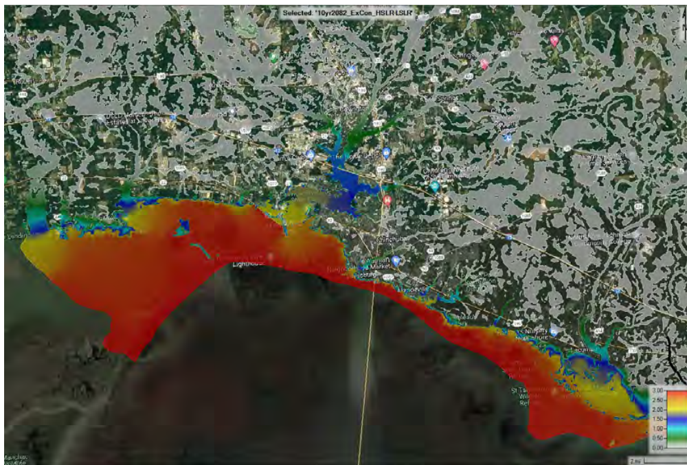
Figure E:14-14. 10-year 2082 event Existing Condition HSLR-LSLR with frequency inflows on the Pearl River and Bogue Chitto River
