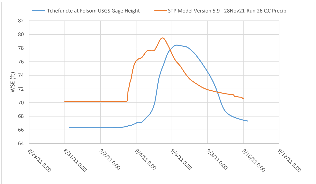
Figure E4.2. September 2011 calibration event plot for USGS Gage -Tchefuncte River at Folsom, LA
