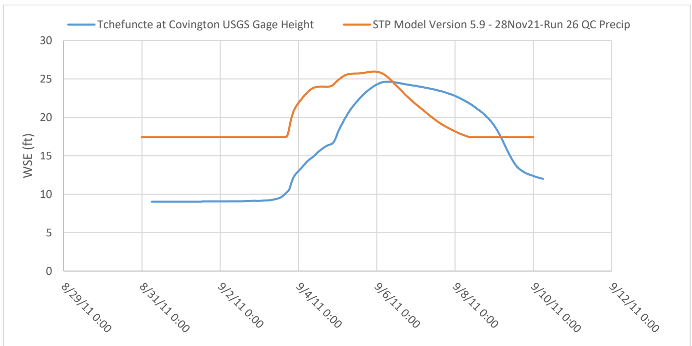
Figure E4.3. September 2011 calibration event plot for USGS Gage -Tchefuncte River at
