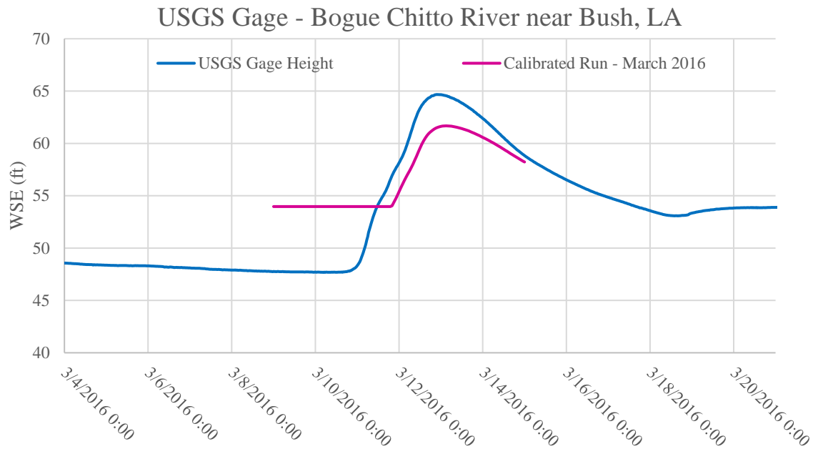
Figure E2:3. March 2016 calibration event plot for USGS Gage -Bogue Chitto River near Bush, LA
