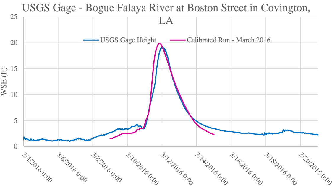
Figure E2:9. March 2016 calibration event plot for USGS Gage -Bogue Falaya River at Boston Street in Covington, LA
