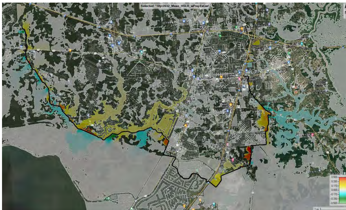
Figure E3:29. 10-year 2032 HSLR difference in WSE with project
