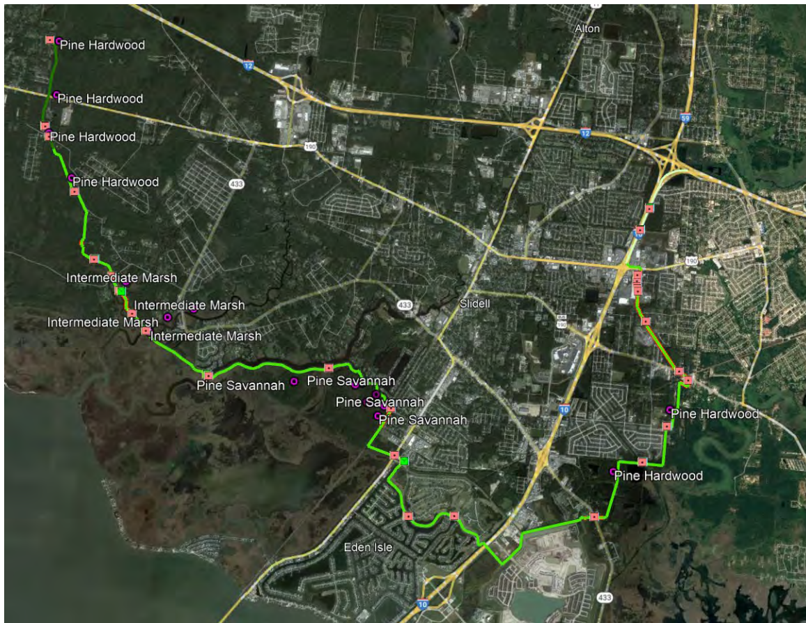
Figure E6:1. Alternative 6c3 Optimized TSP Alignment
