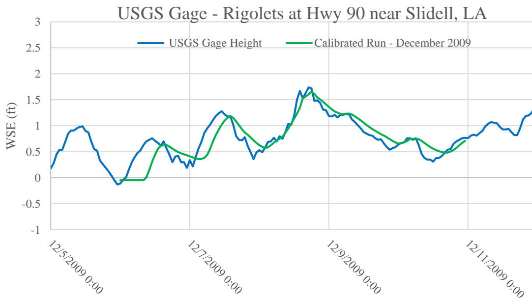
Figure E2:12. December 2009 calibration event plot for USGS Gage -Rigolets at HWY 90
