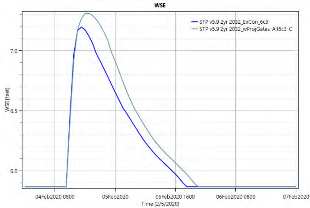
Figure E6:2. Point ID 1 - Pine Hardwood. Point is located on the protected side of the alignment North of Kingspoint Levee. WSE returns to pre-project levels within 36 hours.
