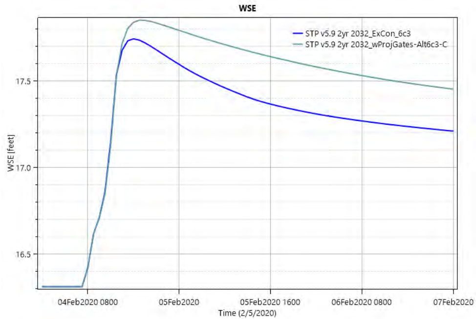
Figure 6:18. Point ID 17 - Pine Hardwood. Point is located on the protected side of the alignment near the Western terminus. WSE remains elevated through the end of the simulation because the drainage path is being obstructed from the North to South. There are no structures in close proximity to this inducement, therefore, a gate was not identified at this location.
