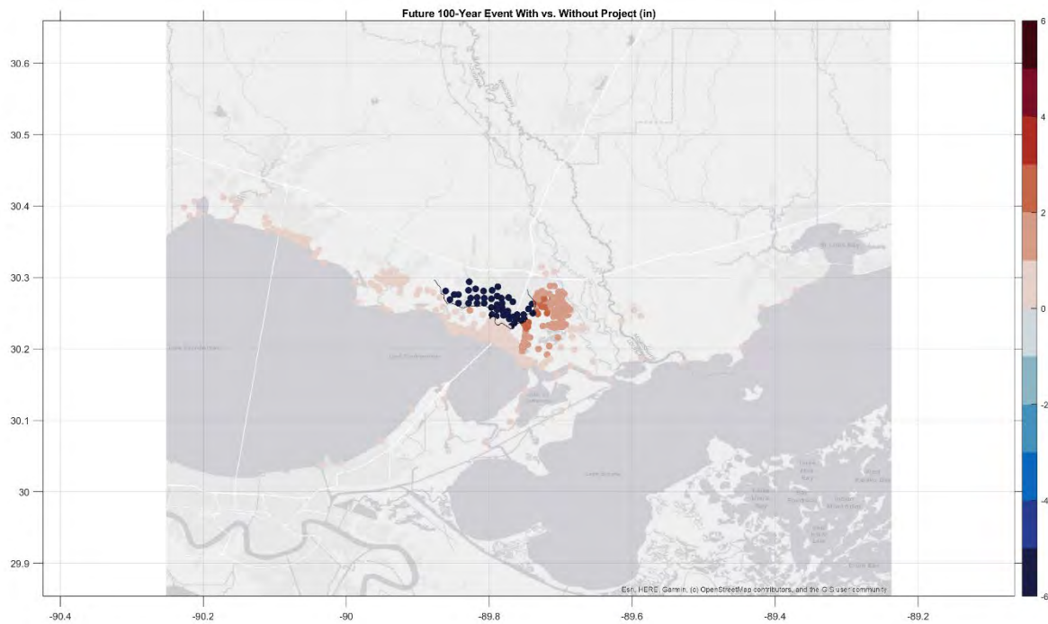
Figure E:13-8. Difference plot of WSE between 2082 with- and without-project values for the 100-year computed WSE (in inches) at various locations surrounding the footprint of the Draft TSP.
