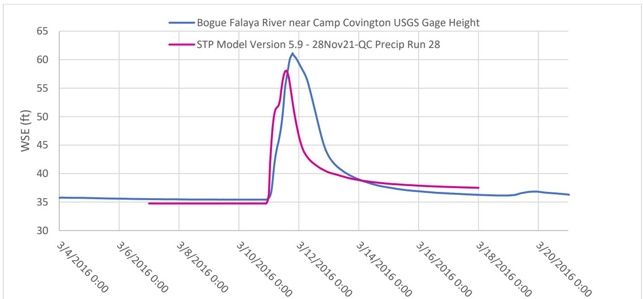
Figure E4:12. March 2016 calibration event plot for USGS Gage – Bogue Falaya River near Camp Covington, LA
