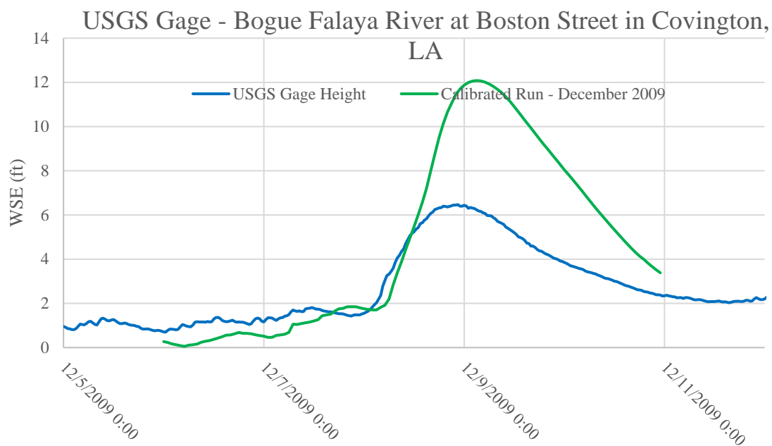
Figure E2:18. December 2009 calibration event plot for USGS Gage -Bogue Falaya River at Boston Street in Covington, LA
