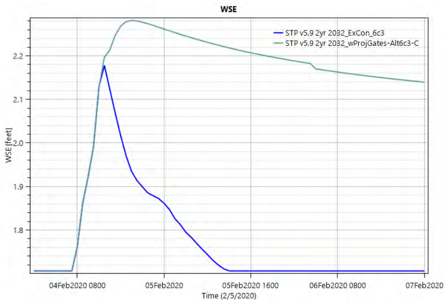
Figure E6:7. Point ID 6 - Pine Savannah. Point is located on the flood side of the alignment West of the Norfolk Southern Railroad. Water in this area moves from South to North and flows into Bayou Bonfouca. WSE remains elevated near the end of the simulation because the levee is obstructing the existing drainage path of water, forcing it to pool on the flood side of the alignment.
