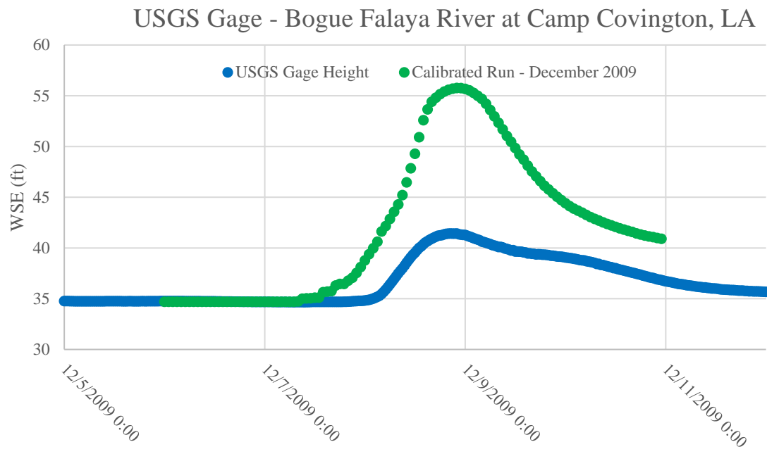
Figure E2:17. December 2009 calibration event plot for USGS Gage -Bogue Falaya River at Camp Covington, LA
