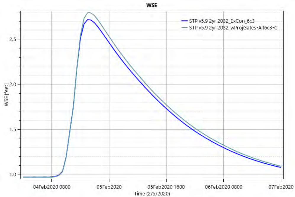
Figure E6:14. Point ID 13 - Intermediate Marsh. Point is located on the protected side of the alignment in the Bayou Paquet floodplain. WSE returns to near pre-project levels by the end of the simulation.
