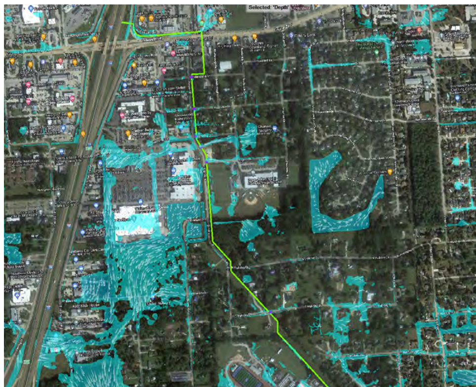
Figure E5:41. Segment 14 Existing Conditions
