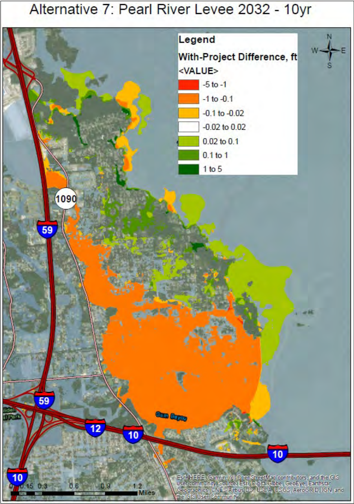
Figure E1:3. Baseline Conditions (year 2032) 10yr frequency event for Pearl River Levee
