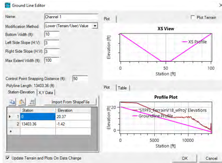
Figure E:14-2. Depiction of channel modification used to apply the Mile Branch channel deepening to the with-project terrain
