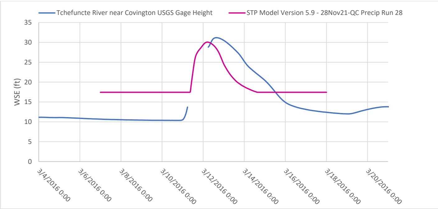
Figure E4:10. March 2016 calibration event plot for USGS Gage – Tchefuncte River near Covington, LA
