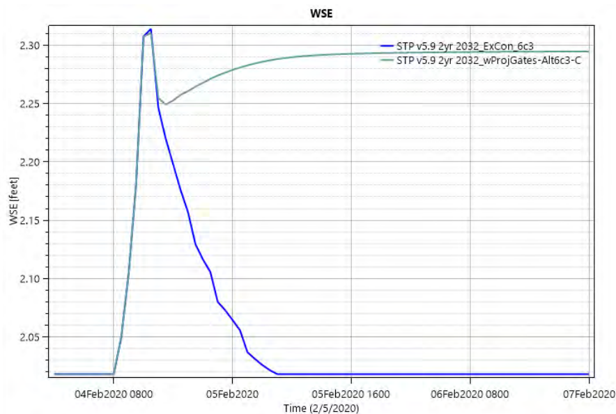
Figure E6:5. Point ID 4 - Pine Savannah. Point is located on the flood side of the alignment West of the Norfolk Southern Railroad. Water in this area moves from South to North and flows into Bayou Bonfouca. WSE remains elevated near the end of the simulation because the levee is obstructing the existing drainage path of water, forcing it to pool on the flood side of the alignment.
