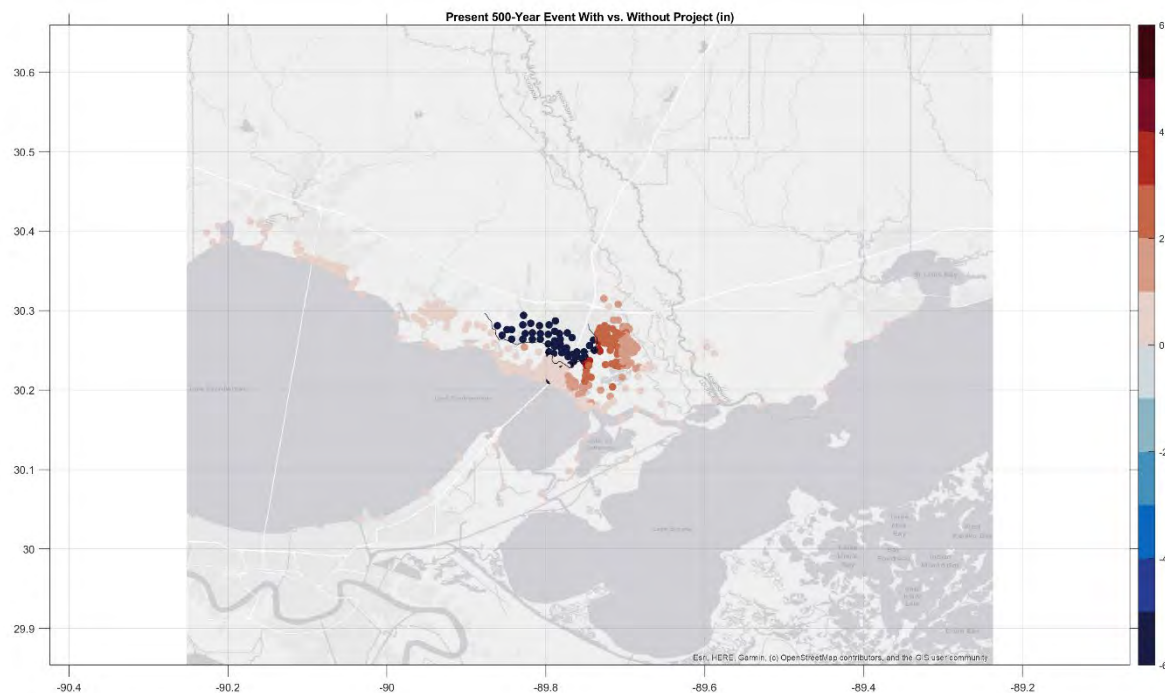
Figure E:13-9. Difference plot of WSE between 2032 with- and without-project values for the 500-year computed WSE (in inches) at various locations surrounding the footprint of the Draft TSP.
