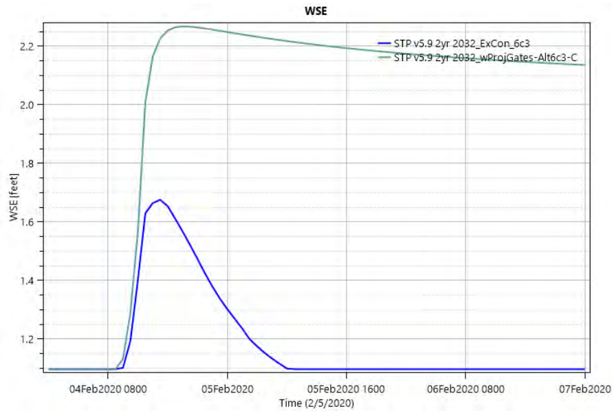
Figure E6:6. Point ID 5 - Pine Savannah. Point is located on the flood side of the alignment West of the Norfolk Southern Railroad. Water in this area moves from South to North and flows into Bayou Bonfouca. WSE remains elevated near the end of the simulation because the levee is obstructing the existing drainage path of water, forcing it to pool on the flood side of the alignment.
