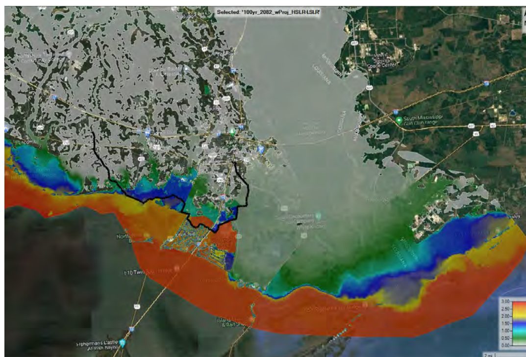
Figure E3:56. 100-year 2082 with-project HSLR minus LSLR
