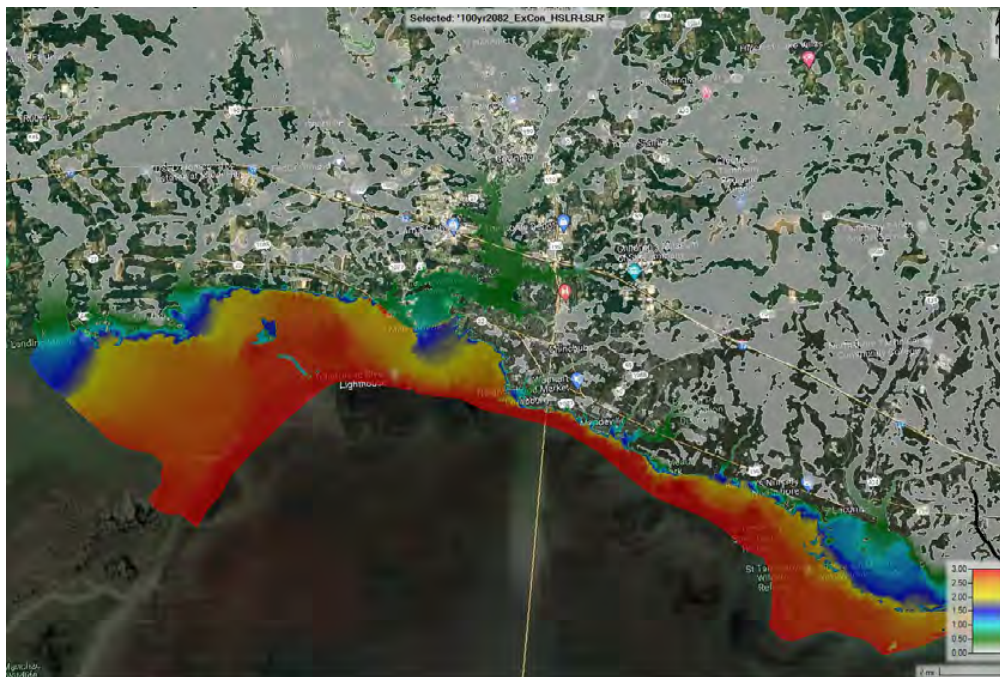
Figure E:14-15. 100-year 2082 event Existing Condition HSLR-LSLR with frequency inflows on the Pearl River and Bogue Chitto River
