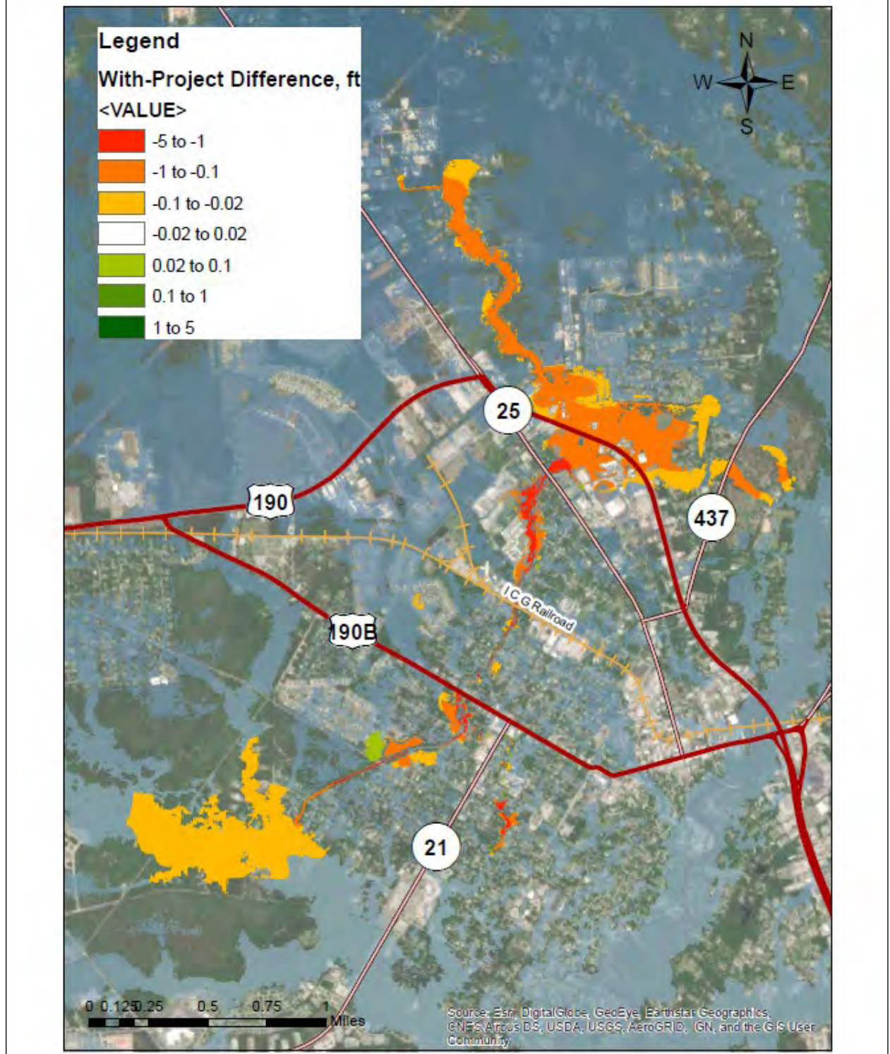
Figure E1:9. Baseline Conditions (year 2032) 10yr frequency event for Mile Branch and Lateral A Dredging
