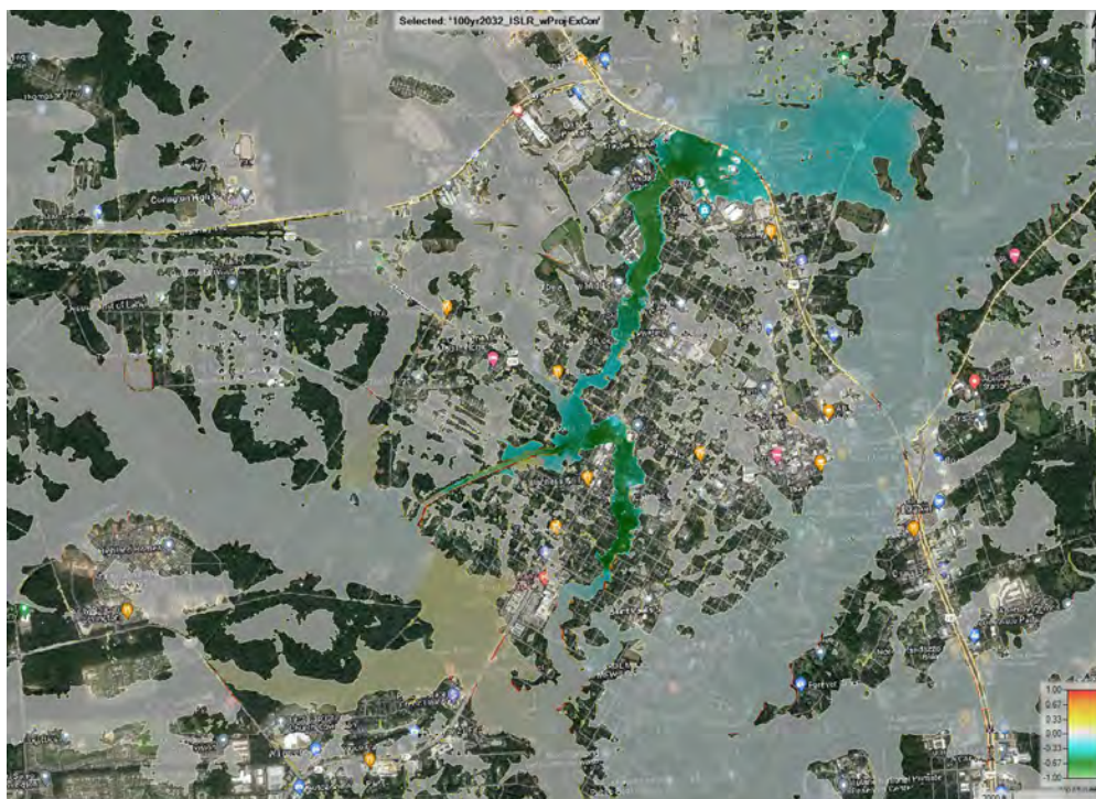
Figure E3:21. 100-year 2032 ISLR difference in WSE with project
