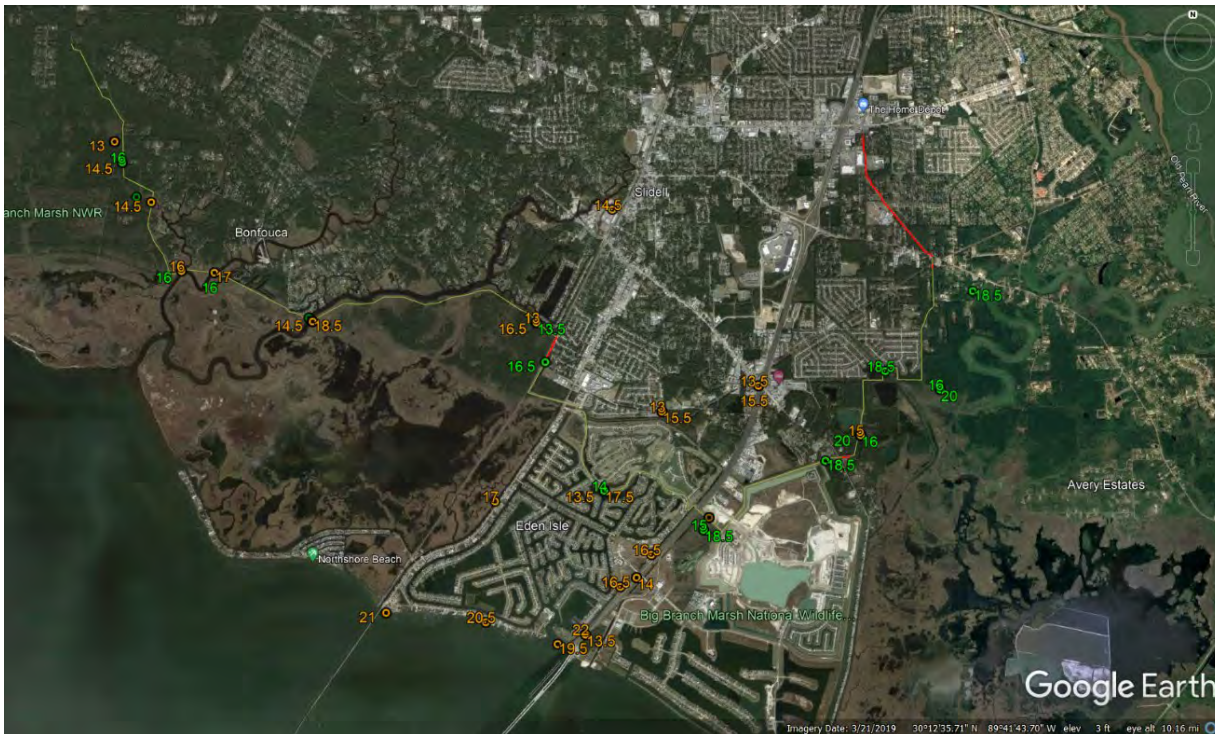
Figure E:13-11. Design heights using prior without-project analysis (orange values) to the updated design heights from the with-project modeling (green values).
