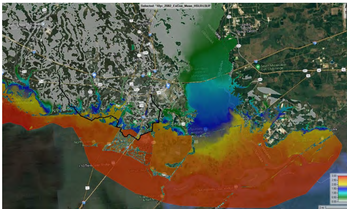
Figure E:14-10. 10-year 2082 event existing conditions HSLR-LSLR with mean inflows on the Pearl River and Bogue Chitto River
