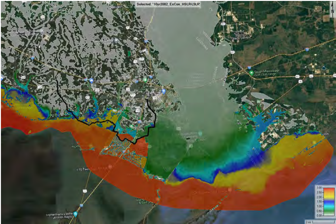
Figure E3:50. 10-year 2082 existing condition HSLR minus LSLR
