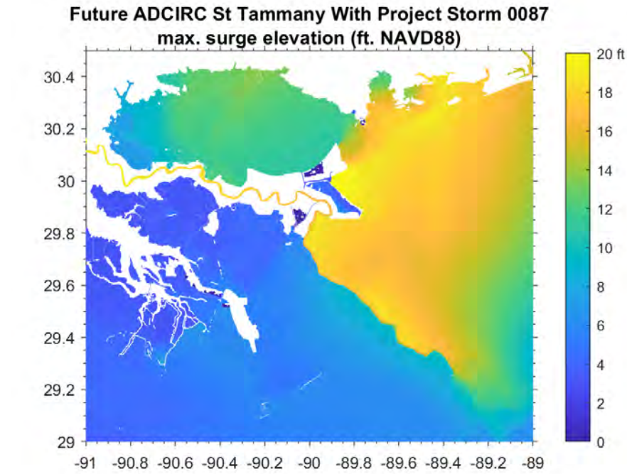
Figure E:13-5. Sample plot of WSE for a future-year with-project simulations from a specific synthetic storm.
