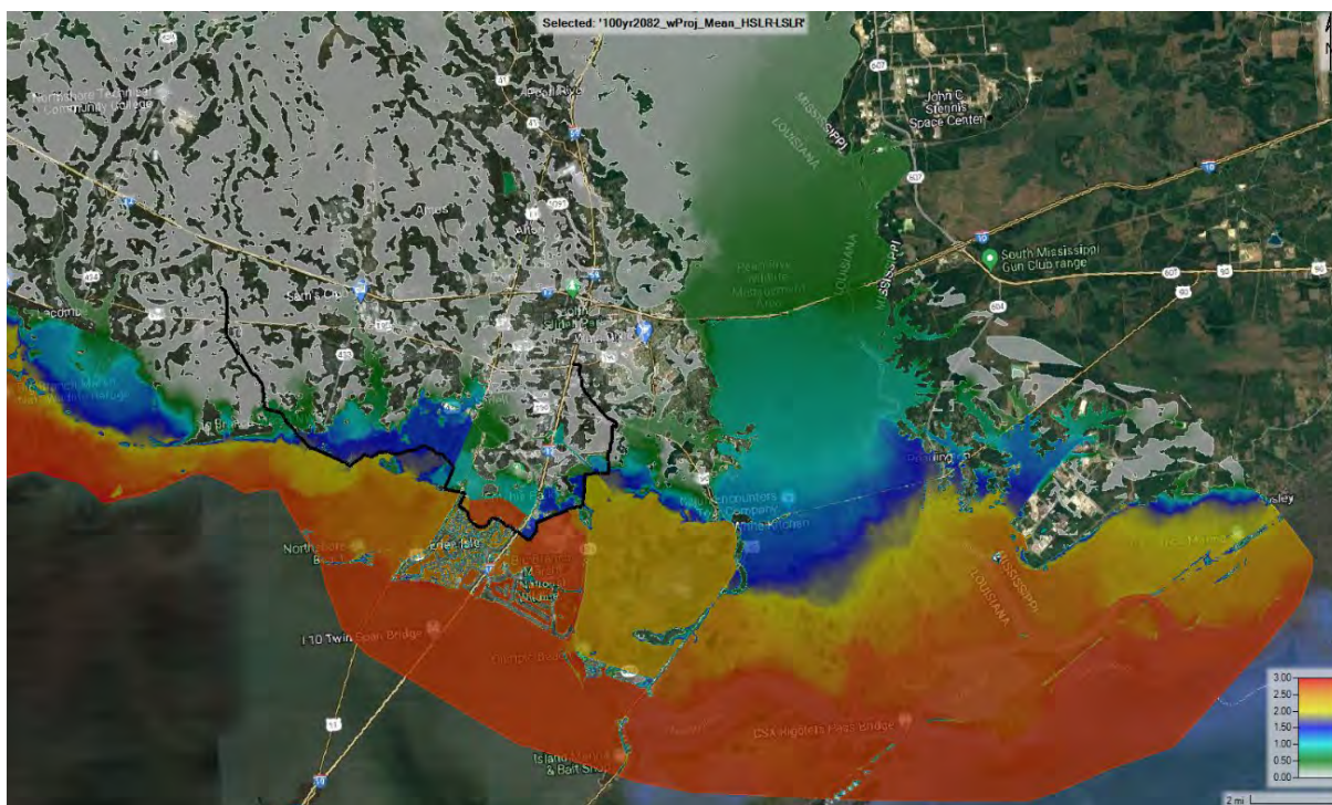
Figure E3:72. 100-year 2082 with-project HSLR minus LSLR
