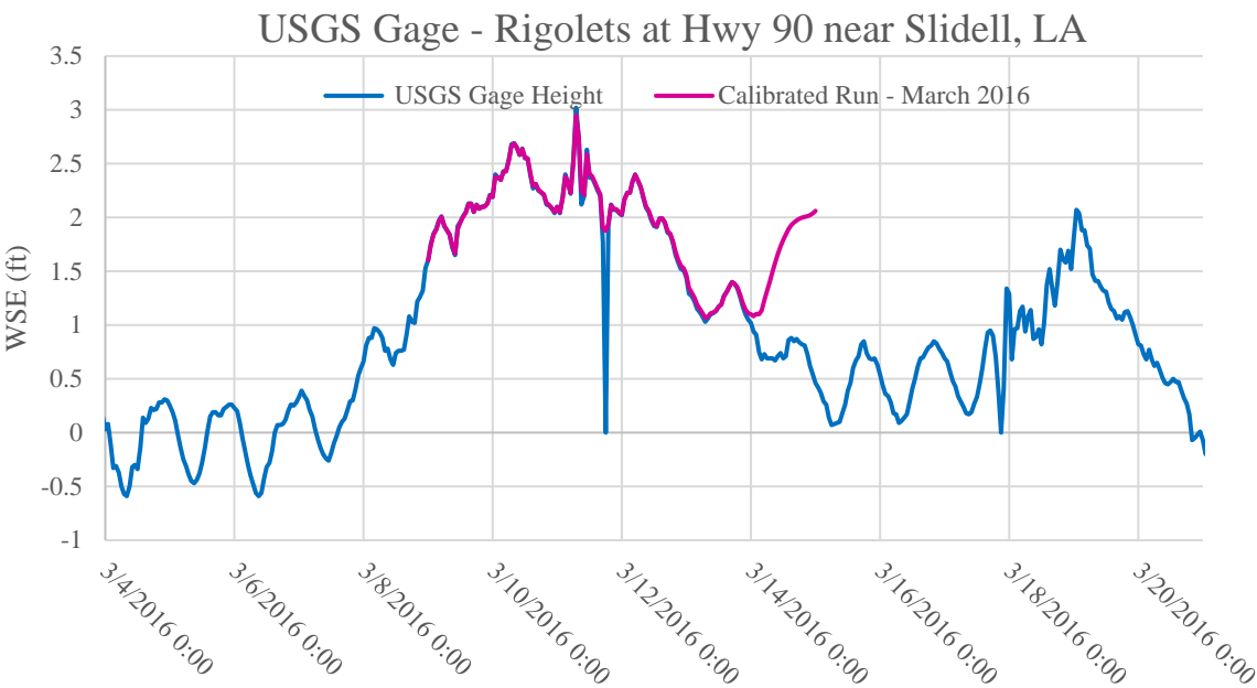
Figure E2:2. March 2016 calibration event plot for USGS Gage -Rigolets at Hwy 90 near Slidell, LA
