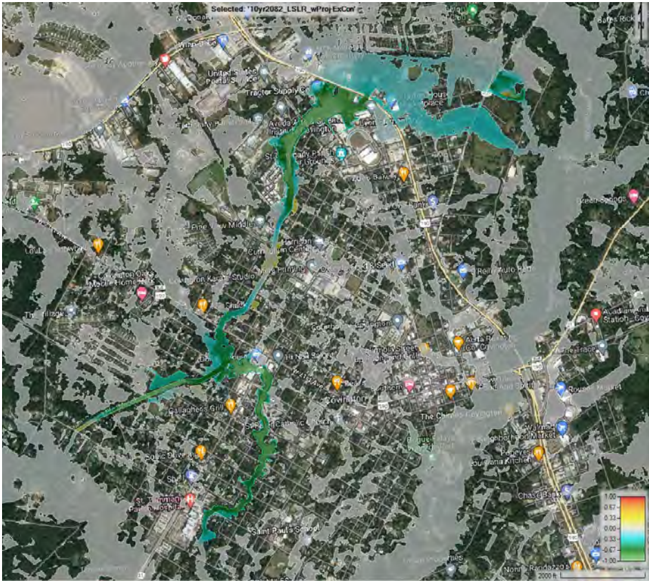
Figure E3.14. 10-year 2082 LSLR difference in WSE with project
