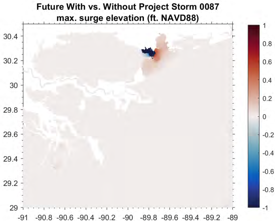
Figure E:13-6. Sample difference plot of WSE between with- and without-project simulations from a specific synthetic storm.
