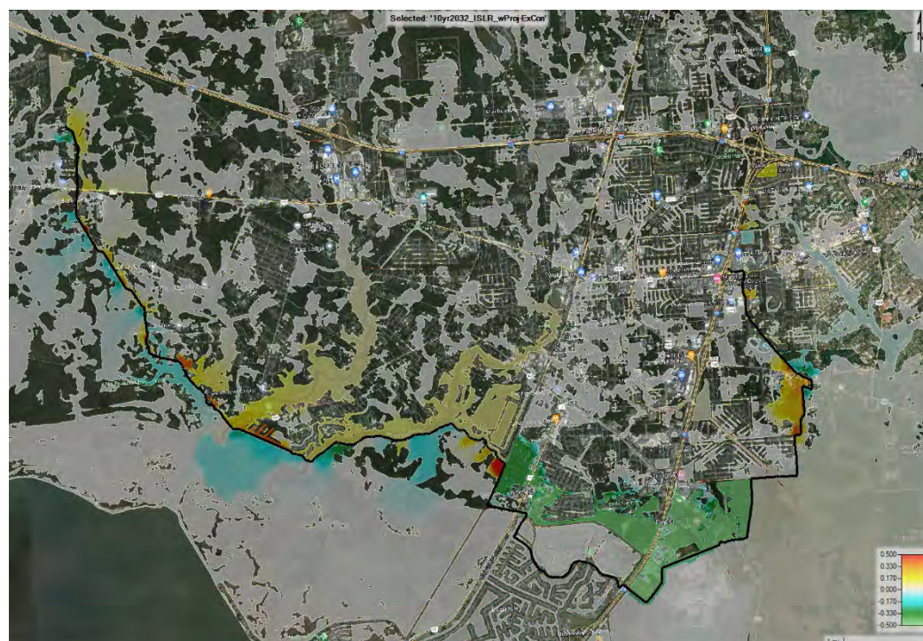
Figure E3.3. 10-year 2032 ISLR difference in WSE with project
