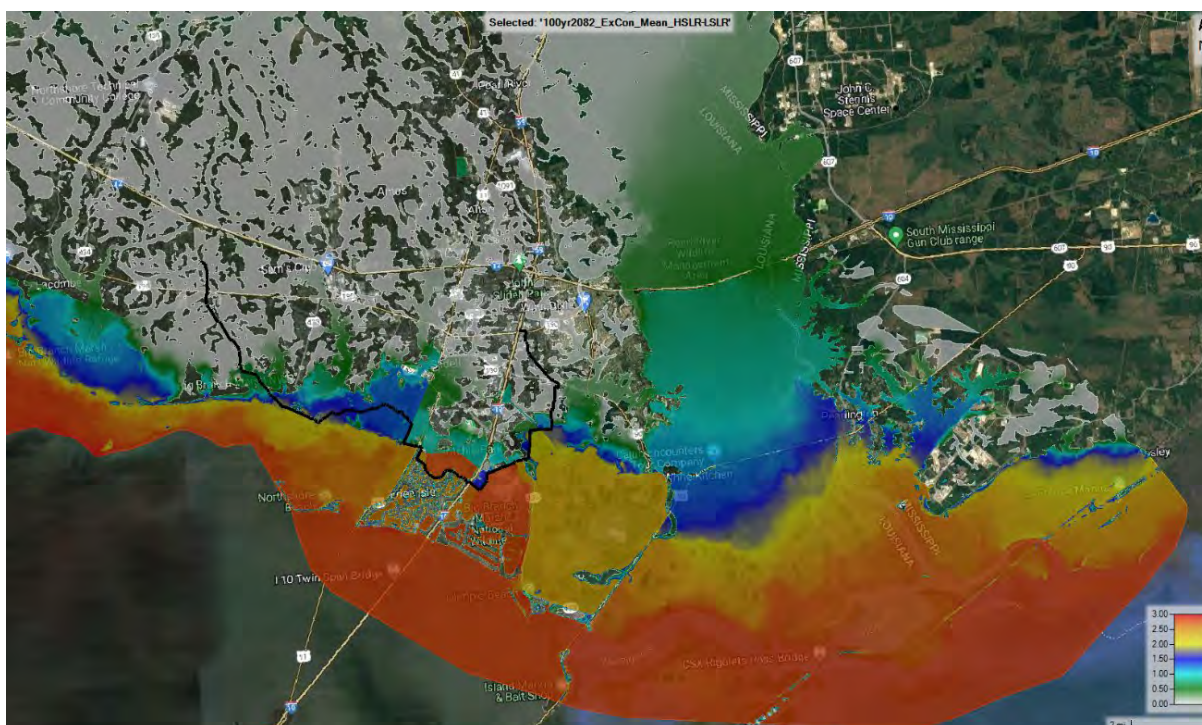
Figure E3:68. 100-year 2082 existing condition HSLR minus LSLR
