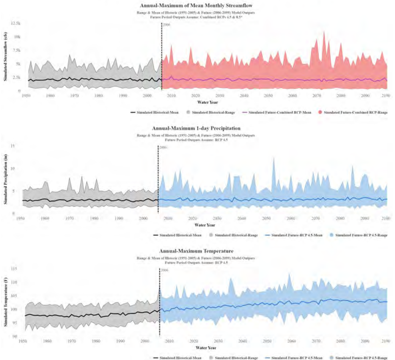
Figure E:11-8. Lower Mississippi River Region 08 CHAT results depicting annual-maximum of mean streamflow, annual-maximum 1-day precipitation, and annual-maximum temperature for the Lower Mississippi HUC-4 basin, Liberty Bayou-Tchefuncte HUC-8 Basin
