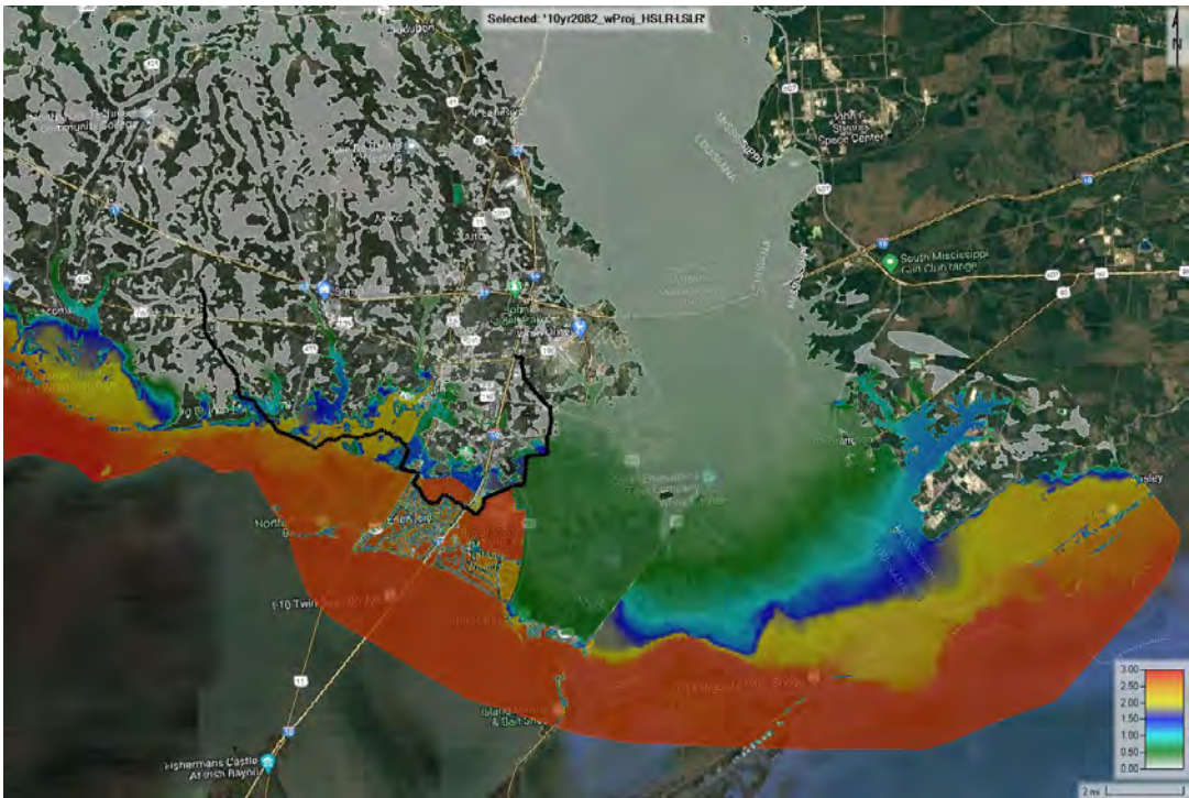
Figure E3:54. 10-year 2082 with-project HSLR minus LSLR
