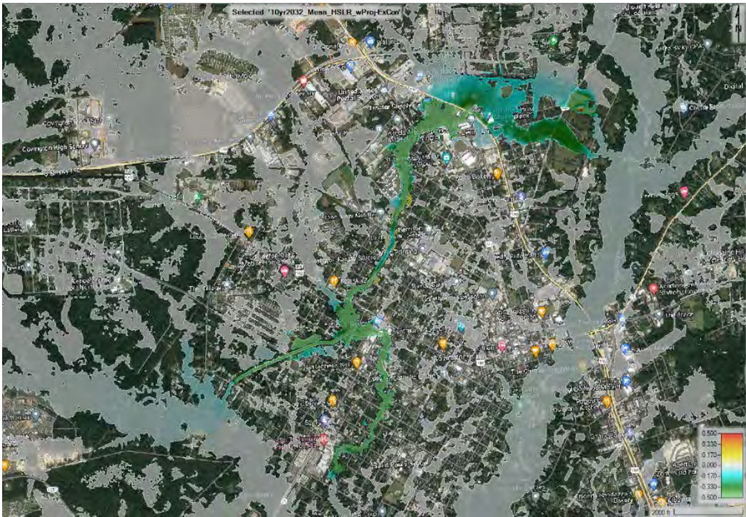
Figure E3:41. 10-year 2032 HSLR difference in WSE with project
