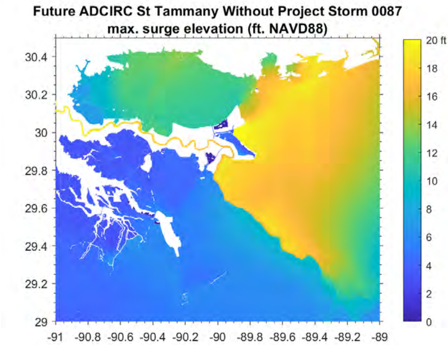
Figure E:13-4. Sample plot of WSE for a future-year without-project simulations from a specific synthetic storm.
