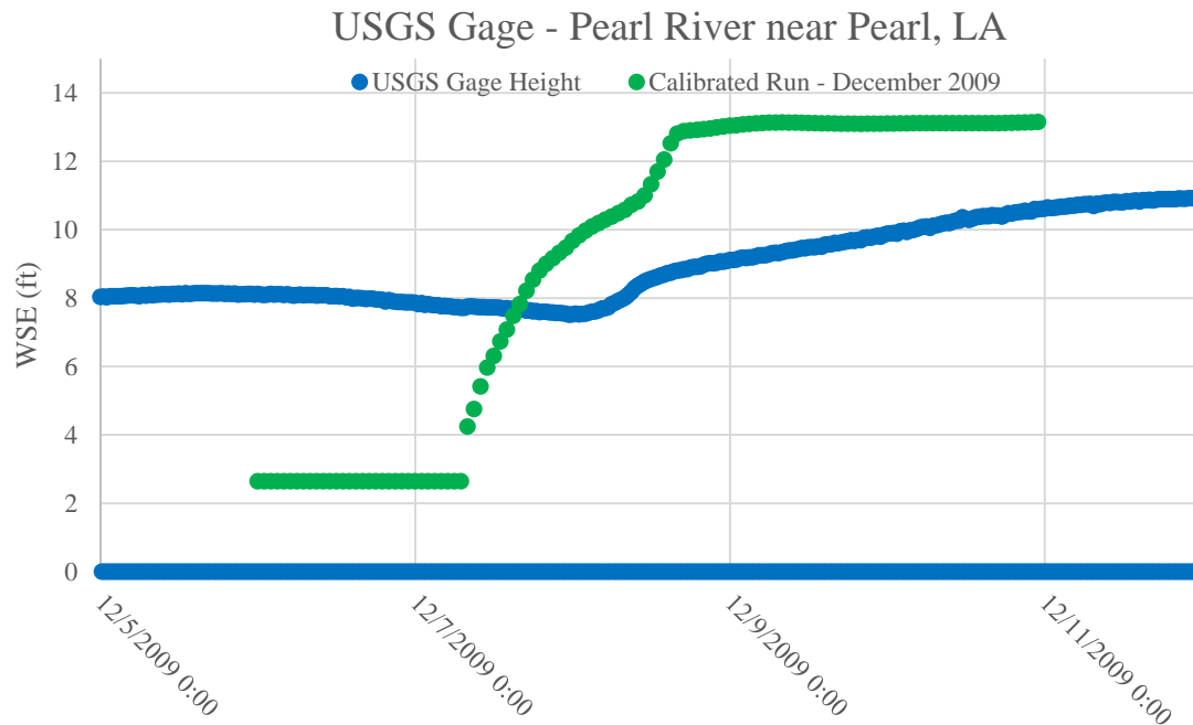
Figure E2:14. December 2009 calibration event plot for USGS Gage -Pearl River near Pearl, LA
