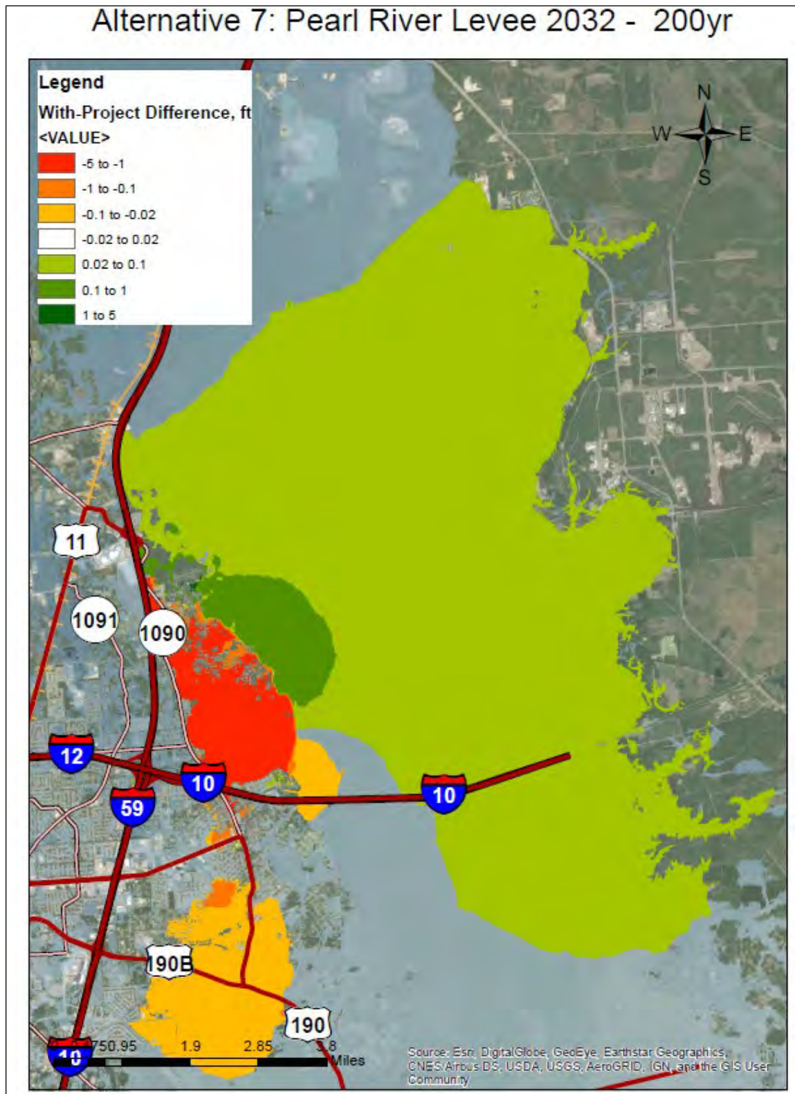
Figure E1:4. Baseline Conditions (year 2032) 200yr frequency event for Pearl River Levee
