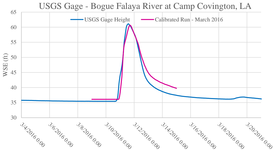
Figure E2:8. March 2016 calibration event plot for USGS Gage -Bogue Falaya River at Camp Covington, LA
