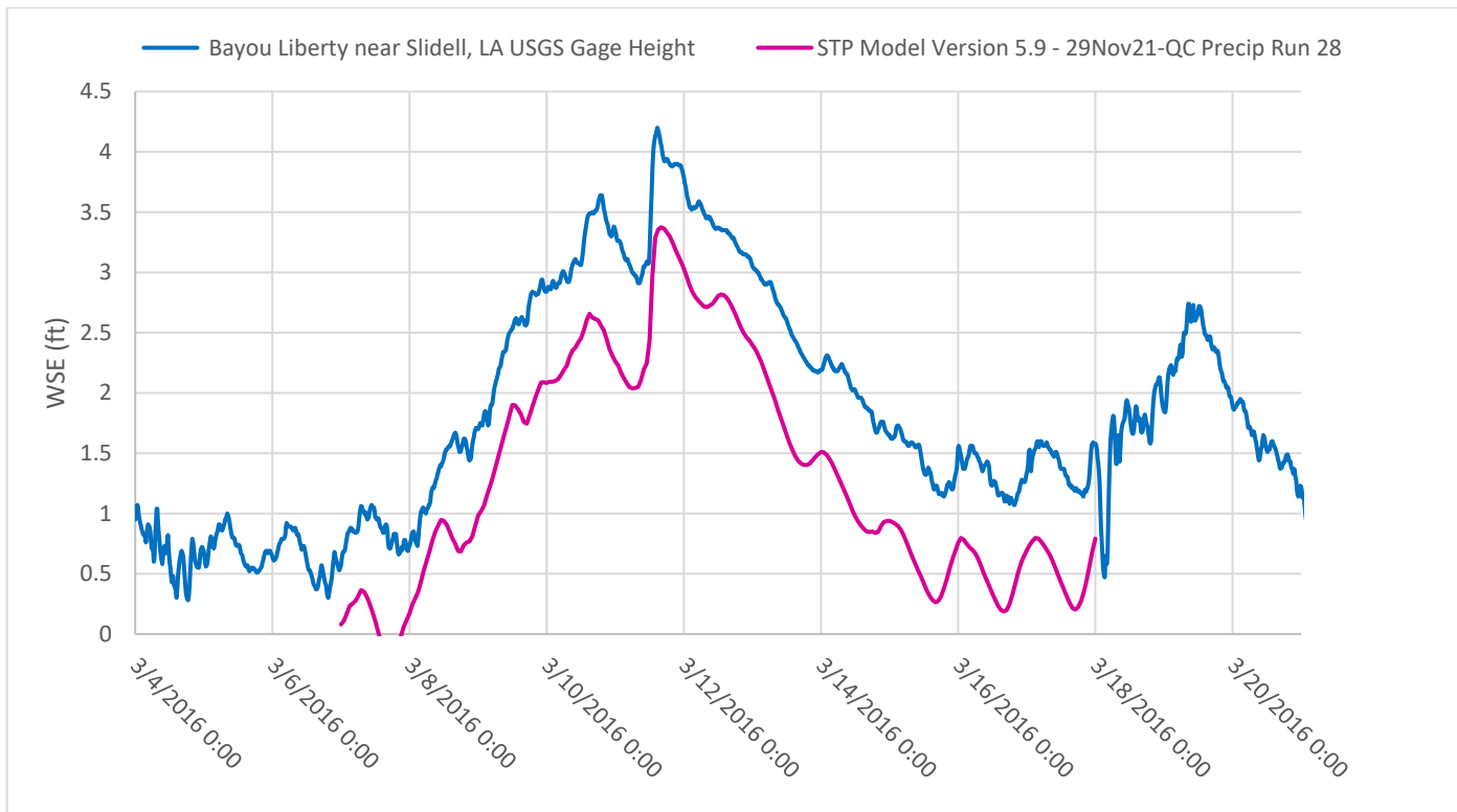
Figure E4:15. March 2016 calibration event plot for USGS Gage – Bayou Liberty near Slidell, LA
