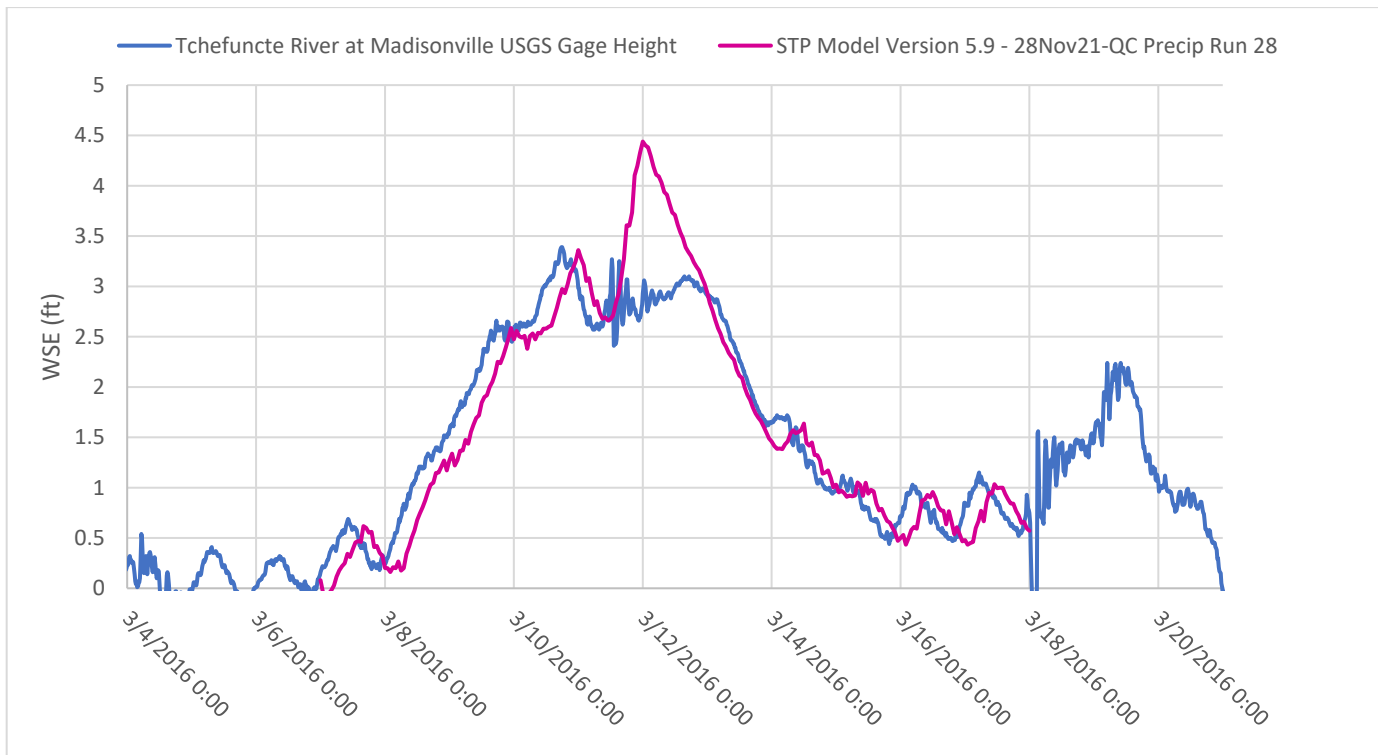
Figure E4:11. March 2016 calibration event plot for USGS Gage – Tchefuncte River at Madisonville, LA
