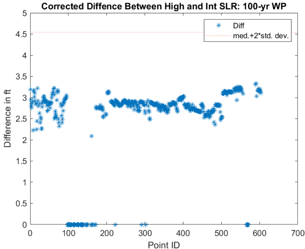
Figure E:13-15. Difference between extrapolated high SLR scenario WSE value and original future intermediate SLR value at a given location with outliers corrected.
