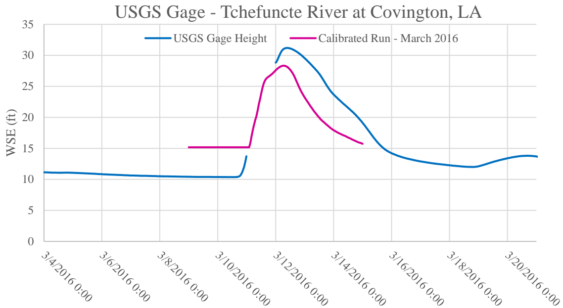
Figure E2:7. March 2016 calibration event plot for USGS Gage -Tchefuncte River at Covington, LA
