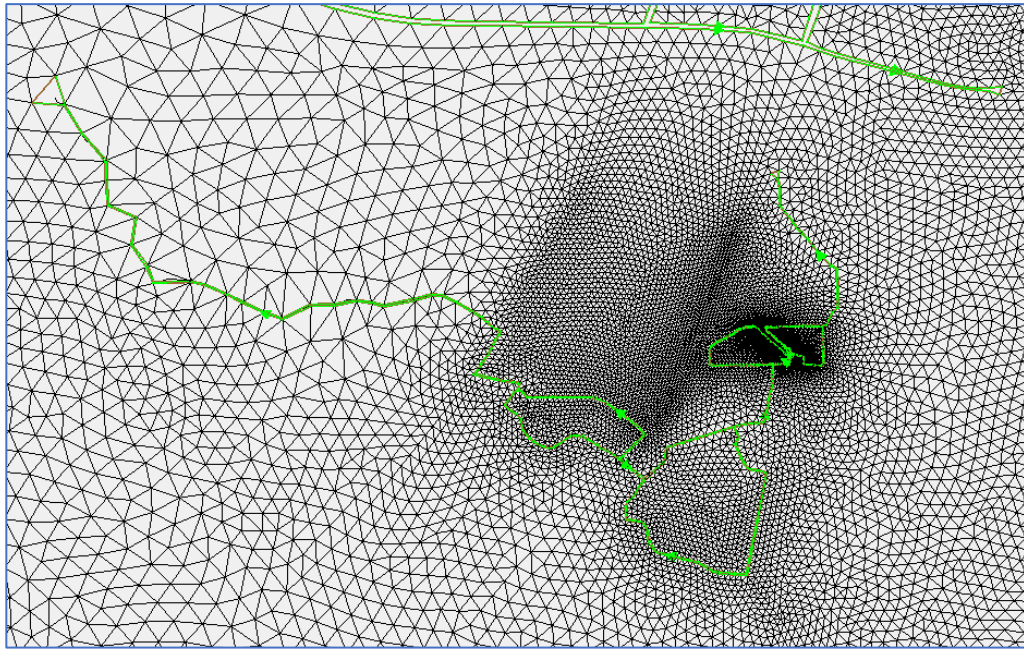
Figure E:13-1. Proposed Draft TSP alignment added to the ADCIRC mesh
