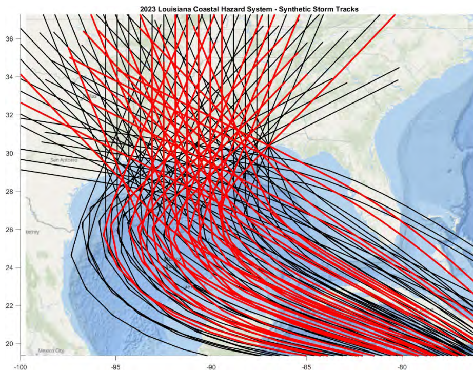
Figure E:13-2. Synthetic storm tracks. Black lines represent the complete suite of 645 storms. Red lines represent the subset of 36 storms simulated with ADCIRC for the STPFS analysis.
