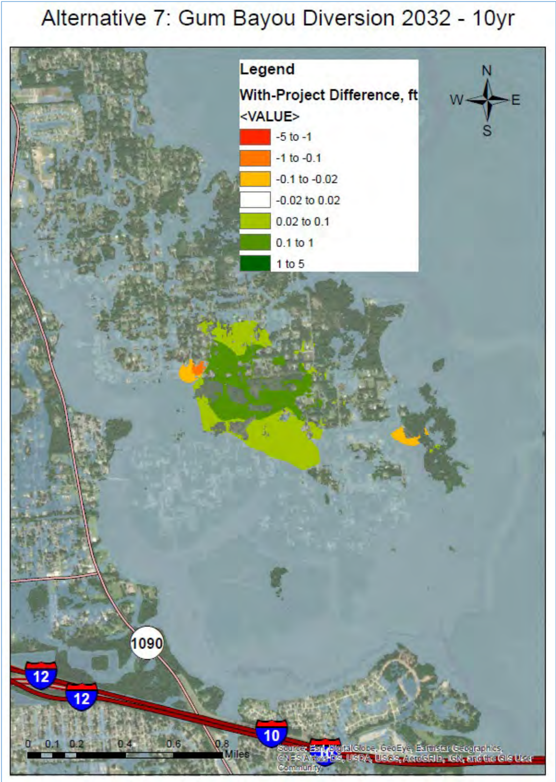
Figure E1:5. Baseline Conditions (year 2032) 10yr frequency event for Gum Bayou
