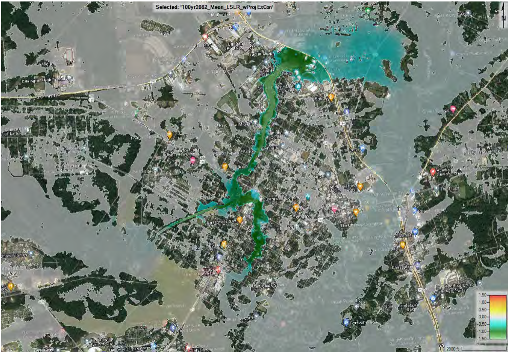
Figure E3:44. 100-year 2082 LSLR difference in WSE with project
