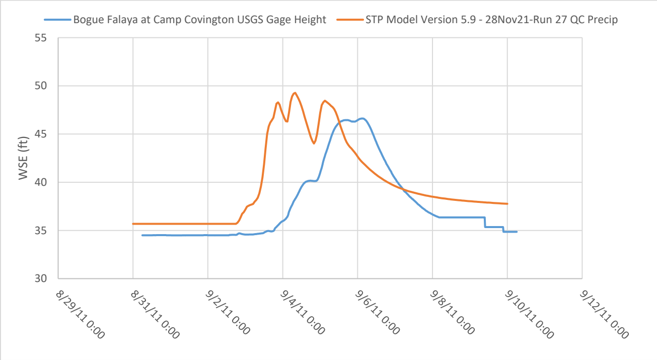
Figure E4:4. September 2011 calibration event plot for USGS Gage -Bogue Falaya at Campe Covington, LA
