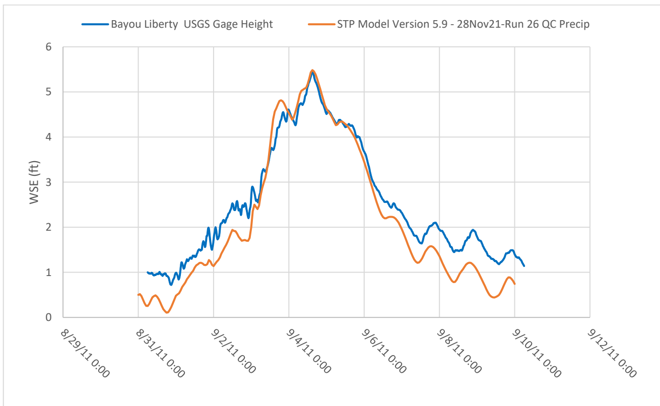
Figure E4:6. September 2011 calibration event plot for USGS Gage -Bayou Liberty
