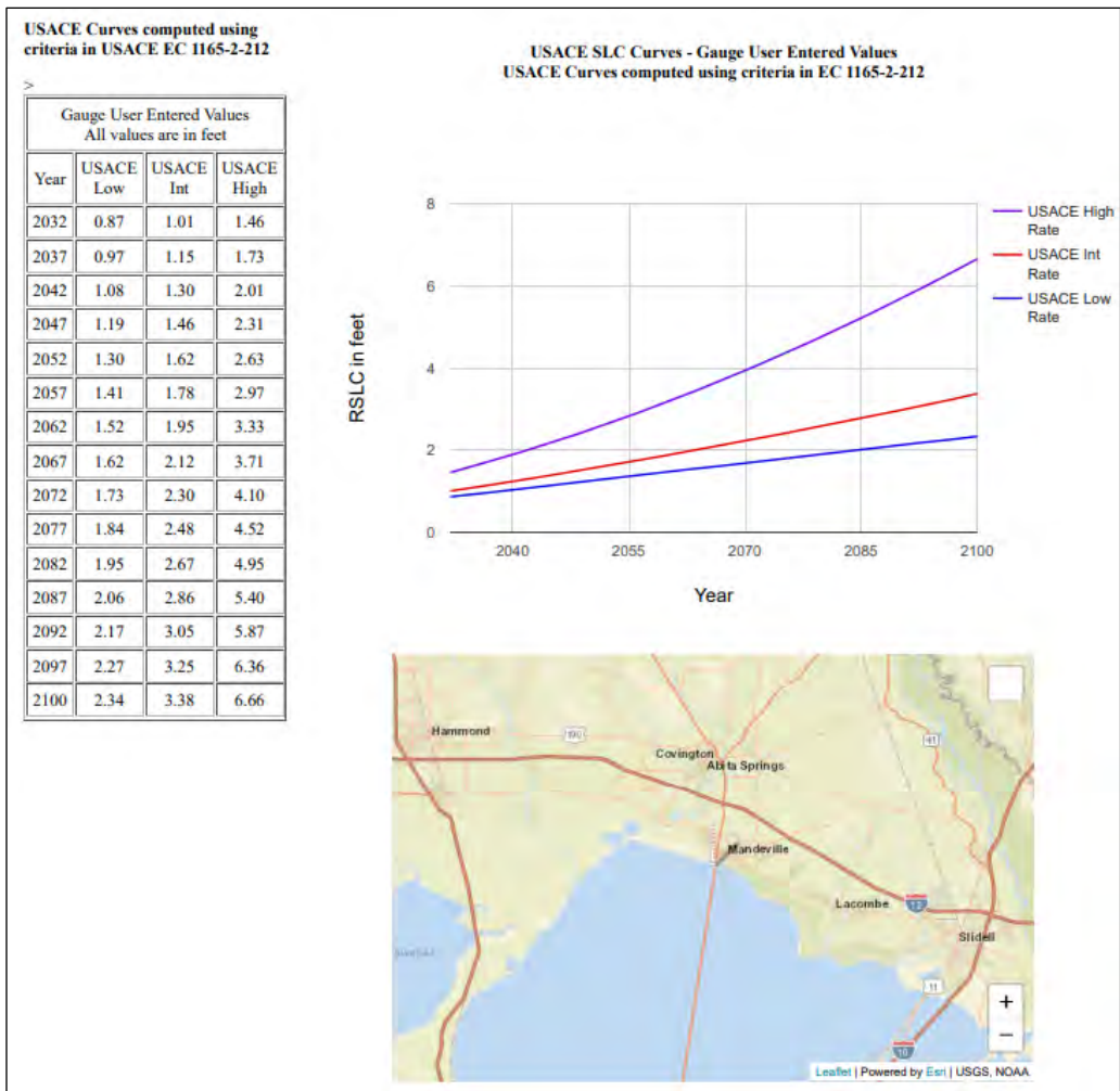
Figure E:3-3. USACE Sea Level Change Curves
