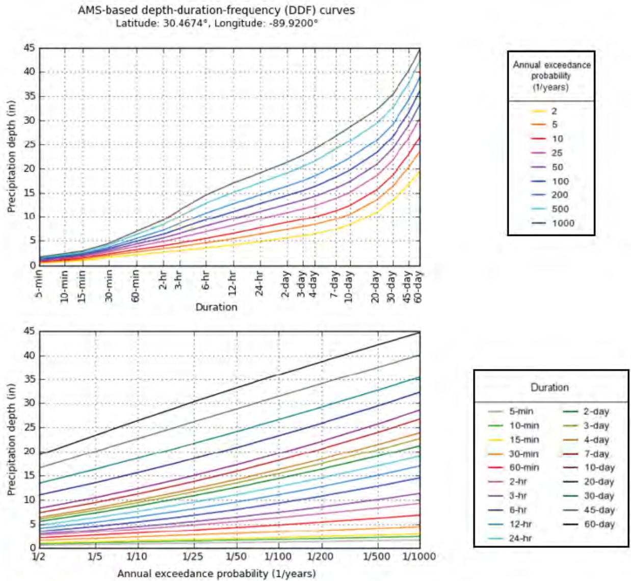
Figure E:10-1. NOAA Atlas 14 Precipitation Data by Annual Exceedance and Duration
