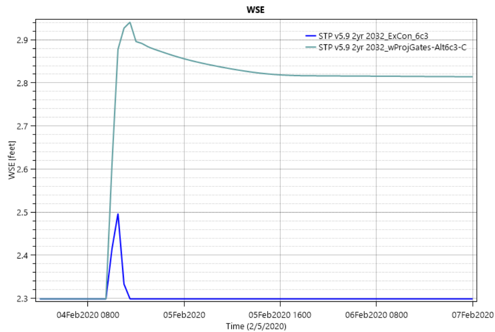
Figure E6:310. Point ID 2 - Pine Hardwood. Point is located on the protected side of the alignment South of Kingspoint Levee. WSE remains elevated through the end of the simulation because an existing drainage path is obstructed. There are no structures in close proximity to this inducement, therefore, a gate was not identified at this location.
