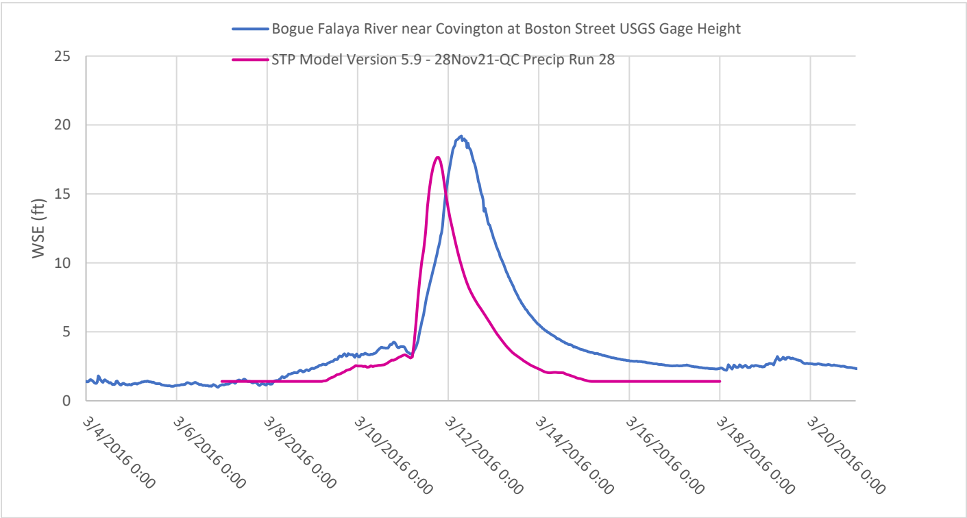
Figure E4:13. March 2016 calibration event plot for USGS Gage – Bogue Falaya River near Covington, LA at Boston Street
