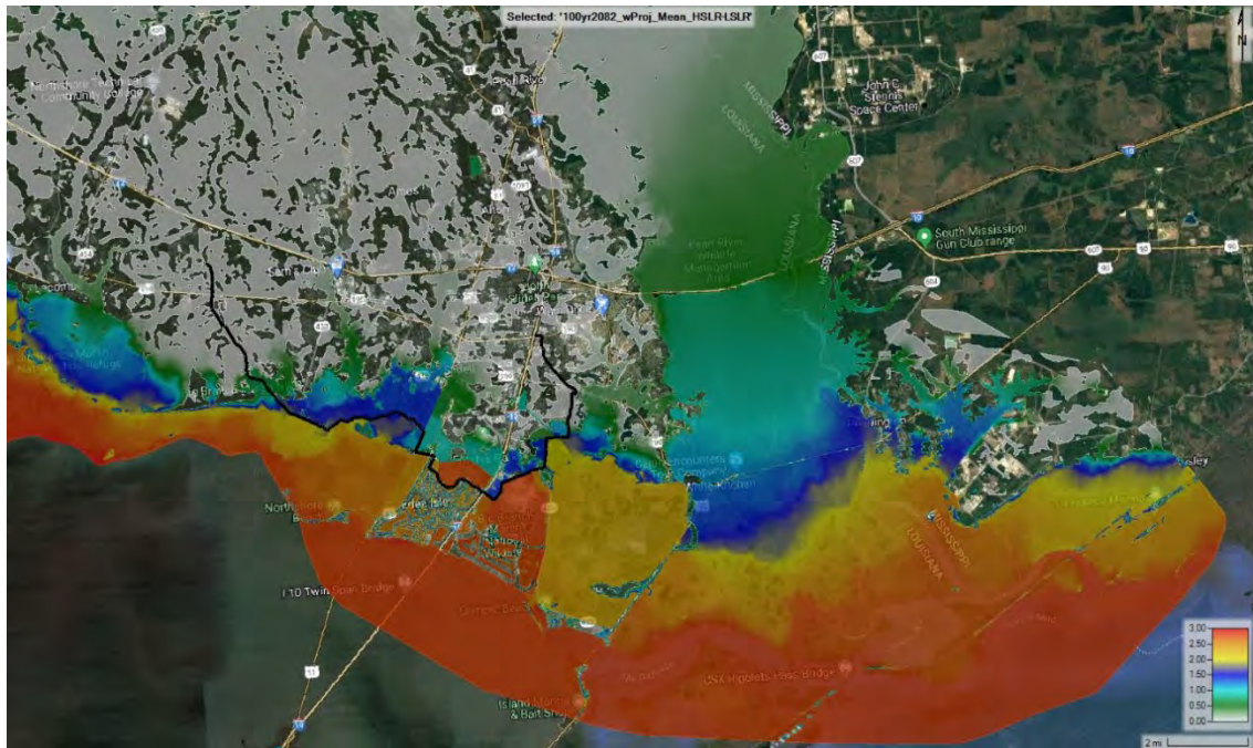
Figure E:14-12. 100-year 2082 event with-project HSLR-LSLR with mean inflows on the Pearl River and Bogue Chitto River
