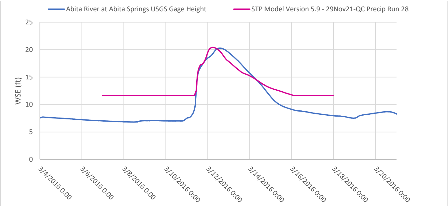
Figure E4:14. March 2016 calibration event plot for USGS Gage – Abita River at Abita Springs, LA
