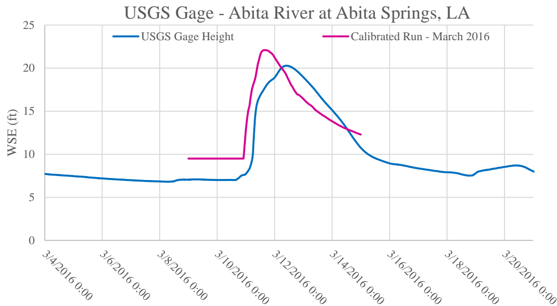
Figure E2:10. March 2016 calibration event plot for USGS Gage -Abita River at Abita Springs, LA
