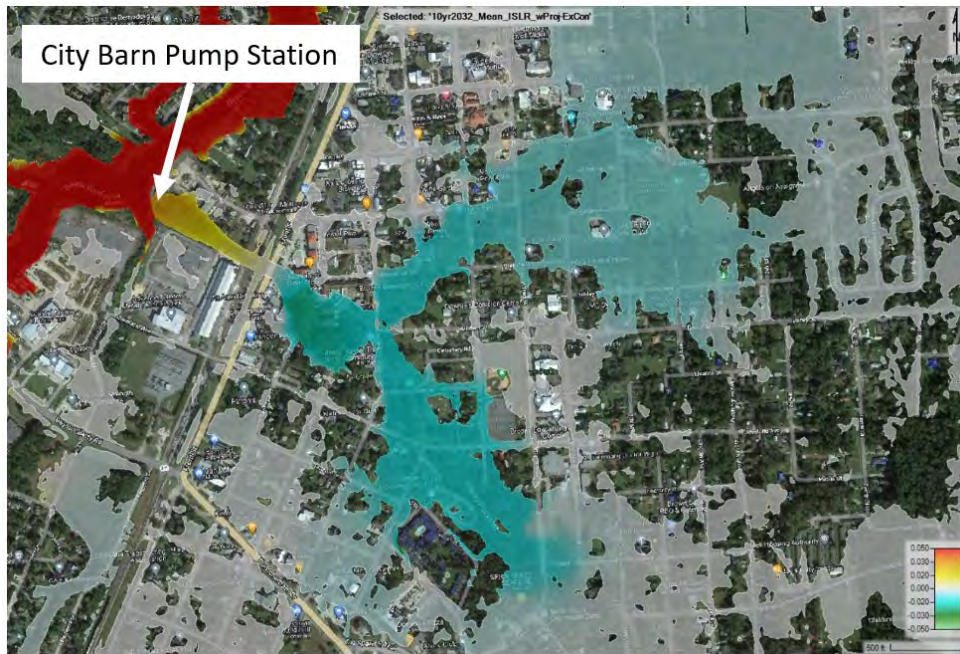
Figure E:14-4. Difference map at Bayou Patassat depicting maximum WSE lowering's with project in place. Blue, green, and cool tones indicate a lowering in WSE in the hundredths range. Red, yellow, and warm tones represent an increase in WSE. Note that there is a pump station at the confluence of Bayou Patassat and Bayou Bonfouca controlling discharge from Bayou Patassat into Bayou Bonfouca called City Barn Pump Station. Inducements exhibited in Bayou Bonfouca are a result of the proposed Levee and scale of the layer, not the Bayou Patassat project.
