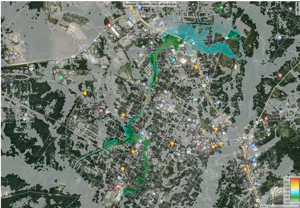
Figure E3:18. 10-year 2082 HSLR difference in WSE with project
