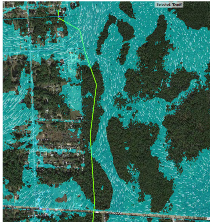
Figure E5:2. Segment 1 Existing Conditions
