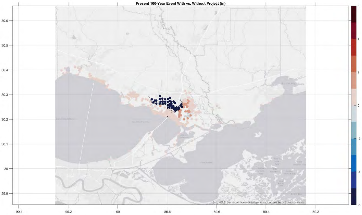
Figure E:13-7. Difference plot of WSE between 2032 with- and without-project values for the 100-year computed WSE (in inches) at various locations surrounding the footprint of the Draft TSP. Blue-colored dots represent reductions with the project in place, on the interior of the proposed system. Red dots represent increases.
