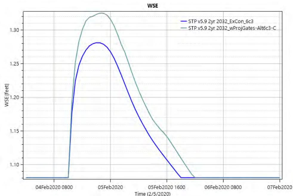
Figure E6:11. Point ID 10 - Intermediate Marsh. Point is located on the protected side of the alignment on the left descending bank of Bayou Liberty. WSE returns to pre-project levels within 36 hours.
