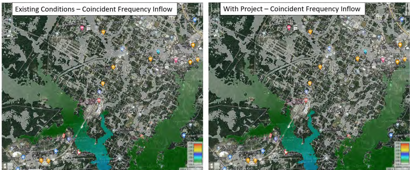
Figure E:14-17. 10-year 2082 event, Existing Condition (left) and With Project (right), depicting the change in WSE between the HSLR-LSLR simulations with coincident frequency inflows on the Pearl River and Bogue Chitto River; zoomed into Mile Branch project area
