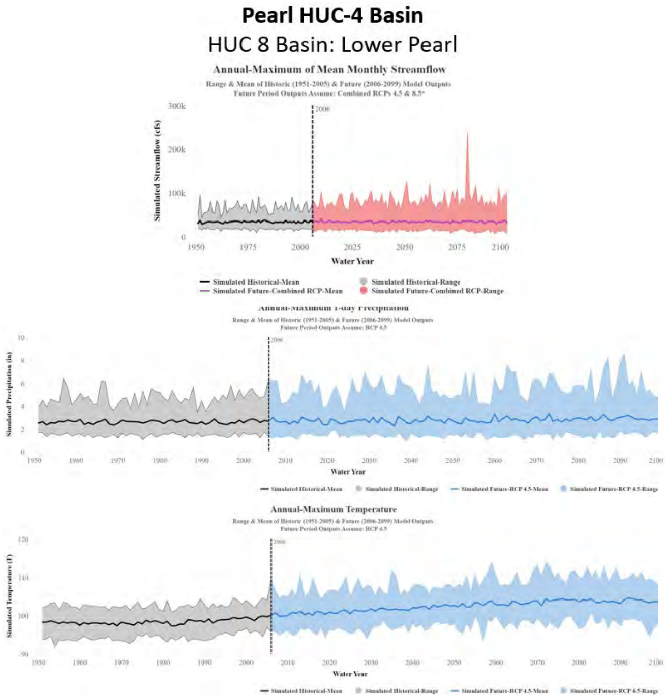
Figure E:11-9. South Atlantic-Gulf Region 03 CHAT results depicting annual-maximum of mean streamflow, annual-maximum 1-day precipitation, and annual-maximum temperature for the Pearl HUC-4 Basin, Lower Pearl HUC-8 Basin
