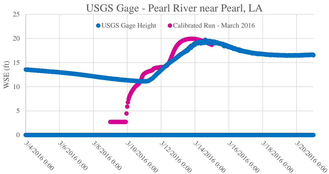
Figure E2:4. March 2016 calibration event plot for USGS Gage -Pearl River near Pearl, LA
